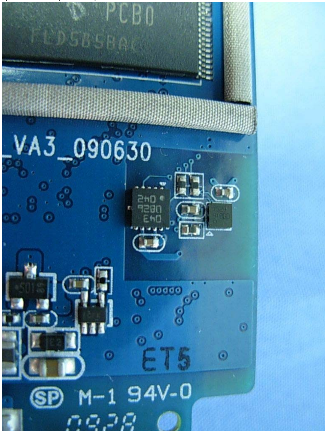
(16) EUT Photo (Wireless)
