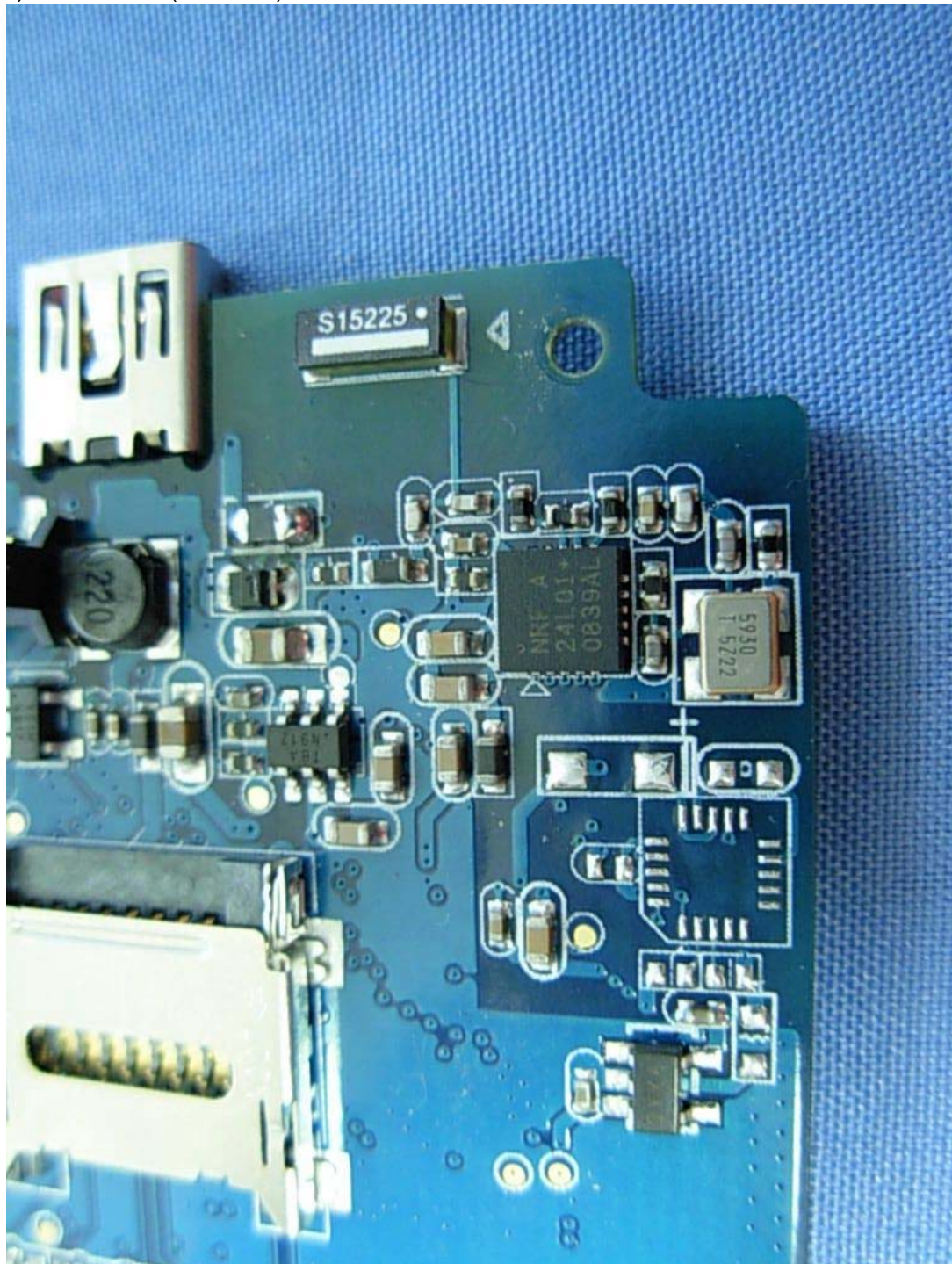
(15) EUT Photo (Wireless)-Antenna
