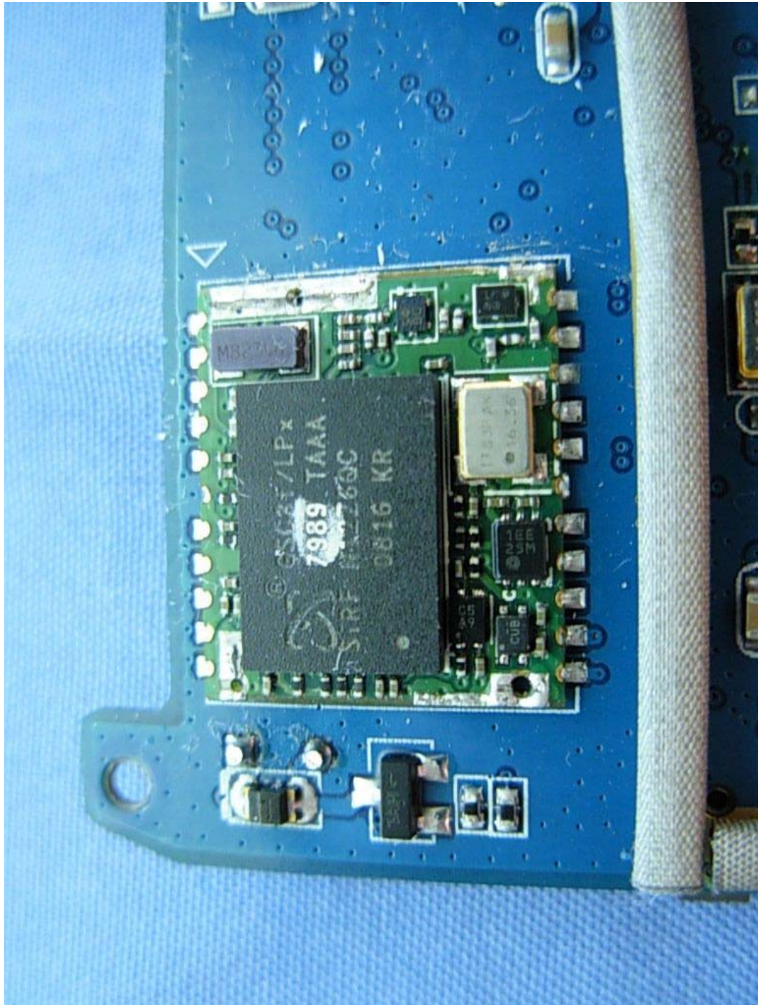
(14) EUT Photo (GPS)
