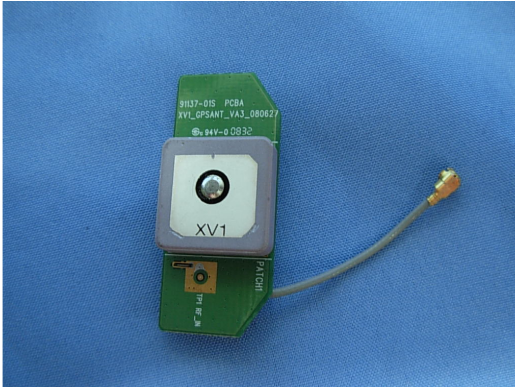
(21) EUT Photo (GPS)-Antenna
