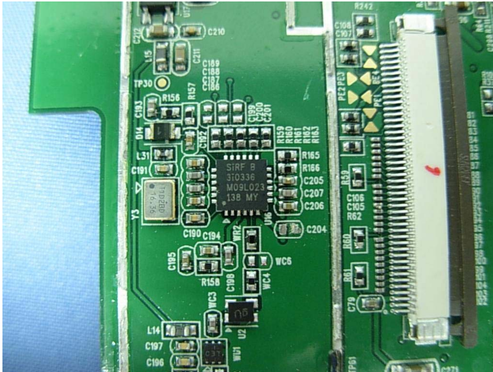
(9) EUT Photo (GPS_MB)
