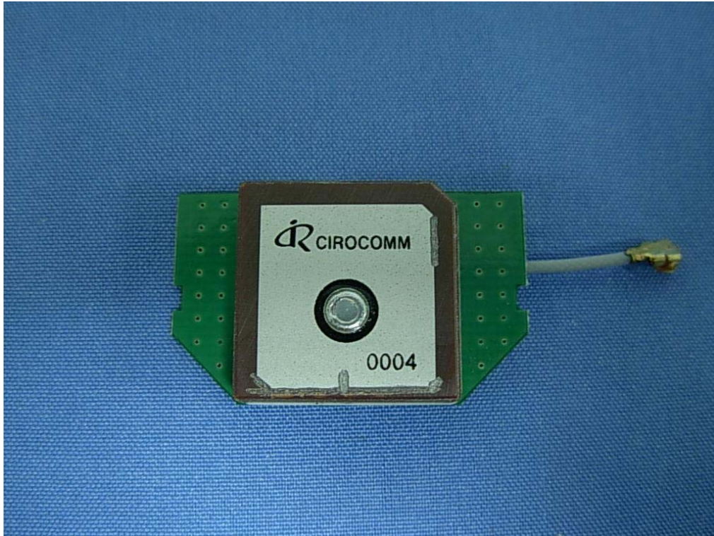
(14)EUT Photo (GPS ANT_1)
