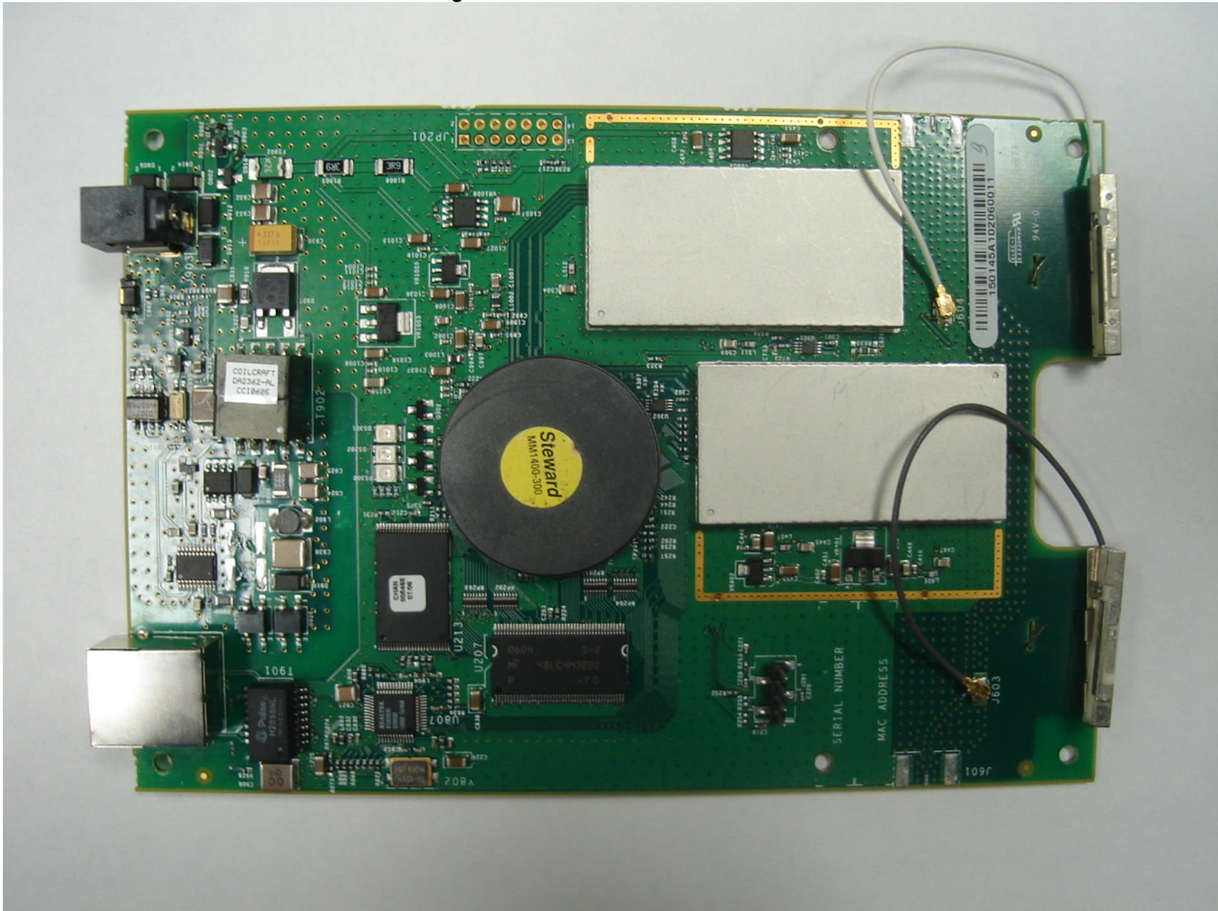
Model Altitude 350-2 Integ 15938 with internal antennas wrt. reversed U.FL connector
