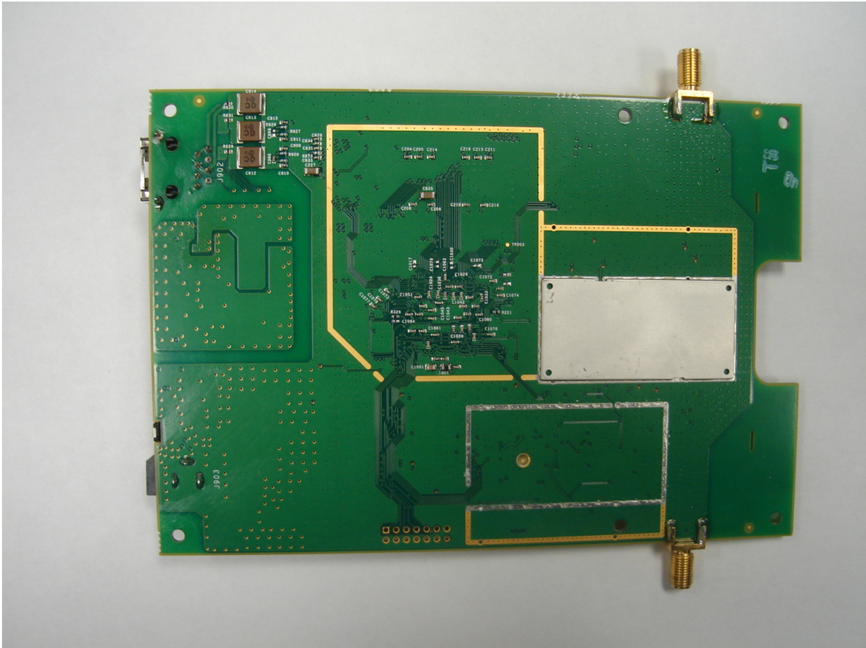
Model ALTITUDE 350-2 DETACH 15939 with external antennas wrt. reversed SMA connector
