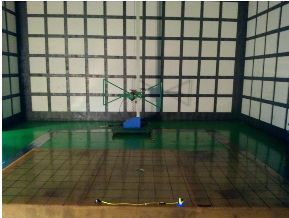
Radiated Emission(30MHz-1000MHz)
