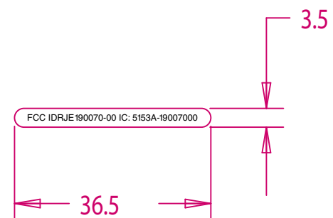
FCC and IC label on Audio Bridge Transmitter unit Model 190070-00
