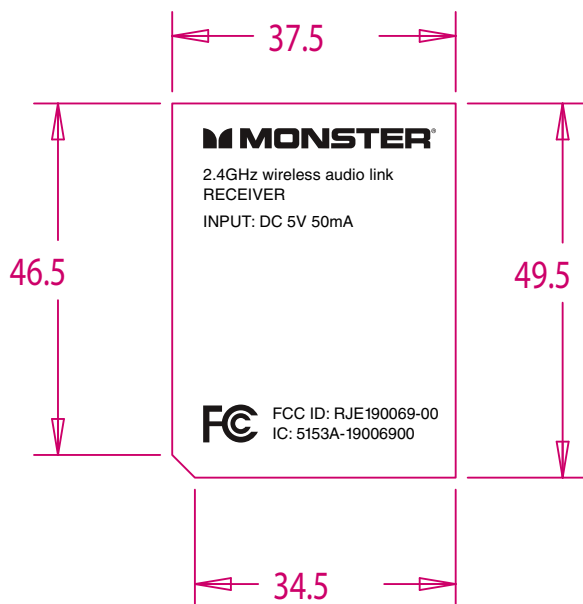
FCC and IC label on Audio Bridge Receiver unit Model 190069-00
