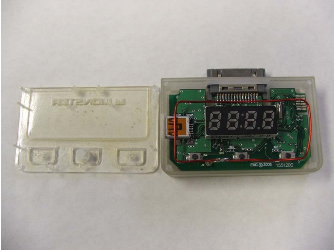
FCC ID: 178065-00 EUT TOP COVER REMOVED
