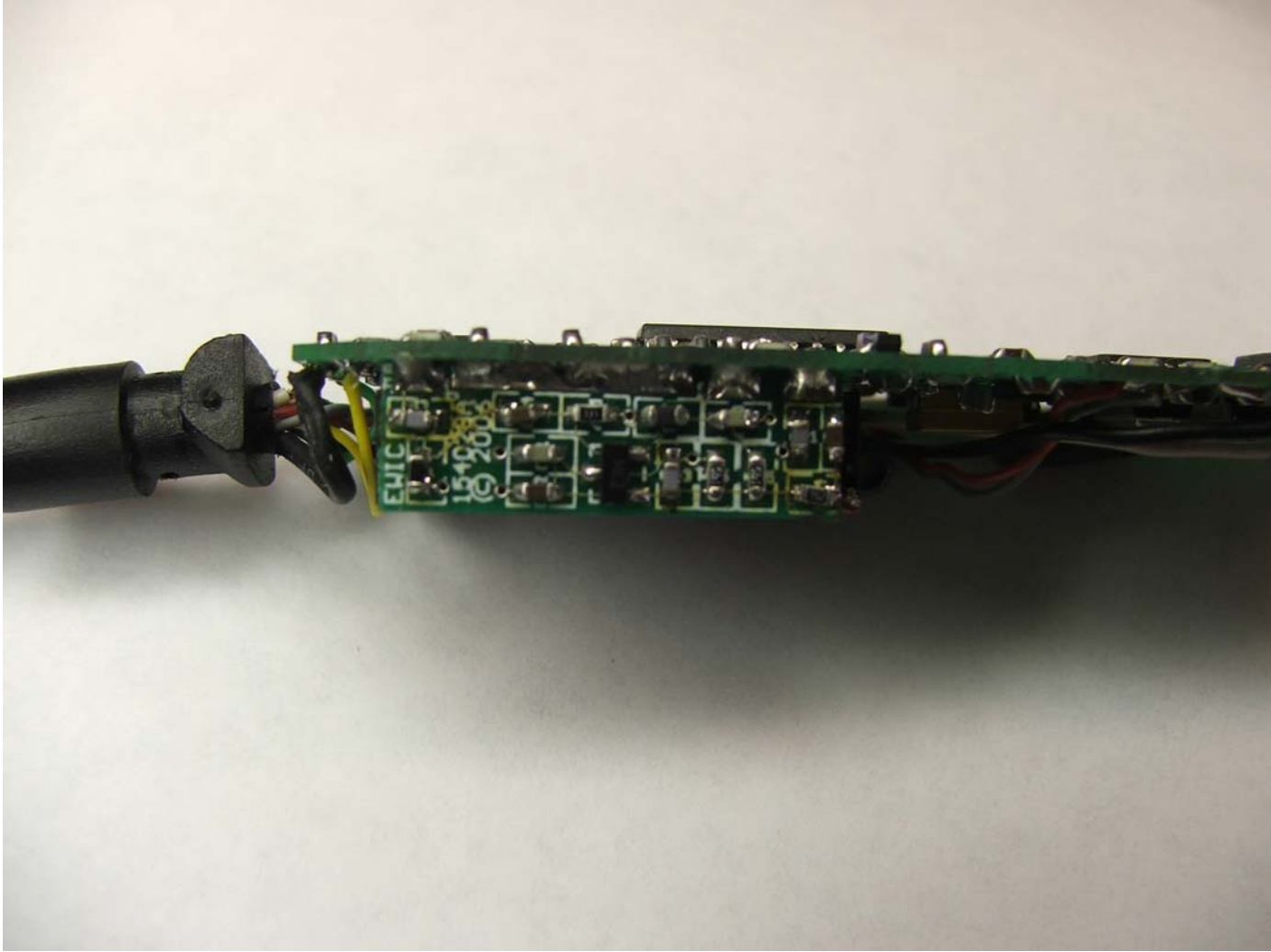
FCC ID: RJE169233-00 LED Display Top PCB
