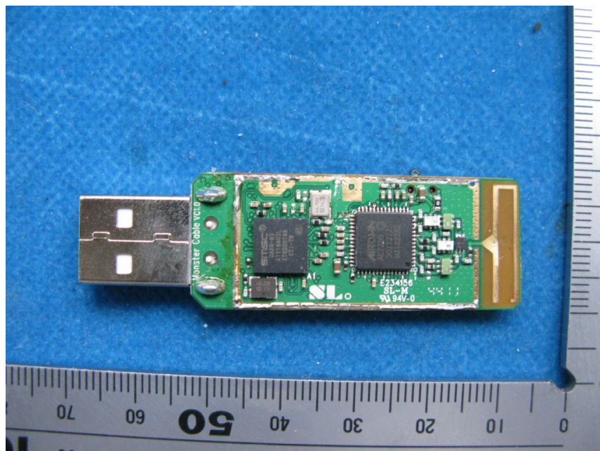
PCB Uncovered View
