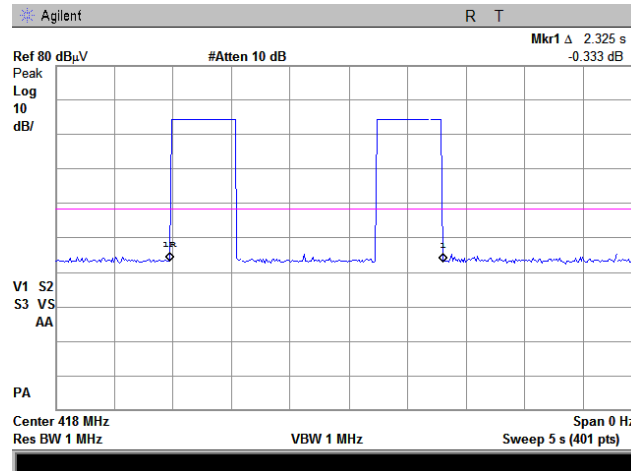
Plot 7.2.23 Transmission train duration
