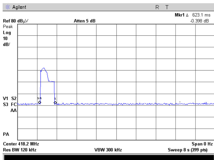
Plot 7.1.1 Transmitter shut down test result - (initialization signal)
