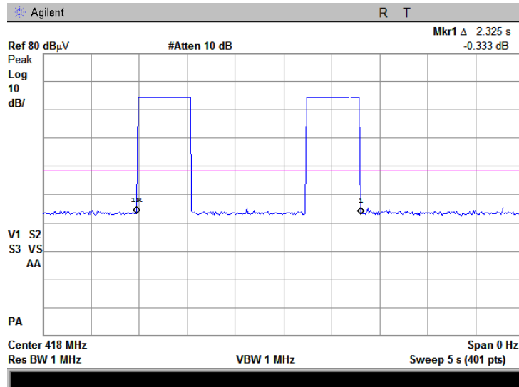
Plot 7.1.4 Alarm detection transmission duration, includes 2 bursts
