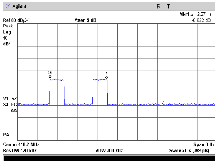
Plot 7.1.2 Transmitter shut down test result - (tamper open signal)
