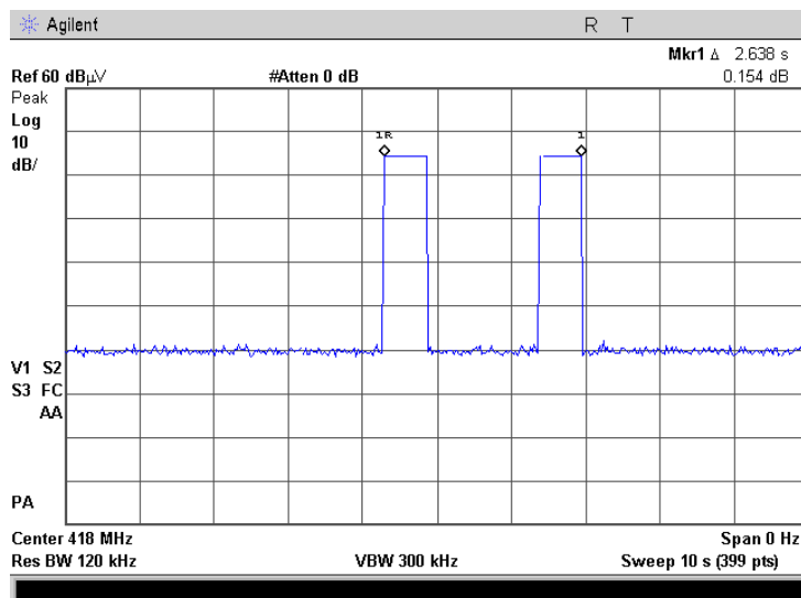
Plot 7.1.3 Transmitter shut down test result (tamper closed signal)
