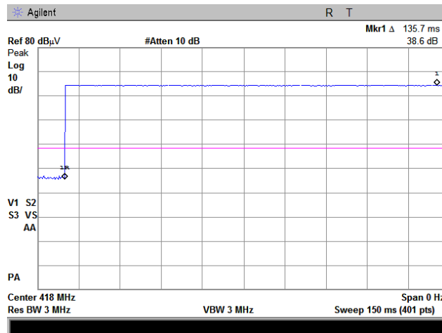
Plot 7.2.20 Transmission pulse duration
