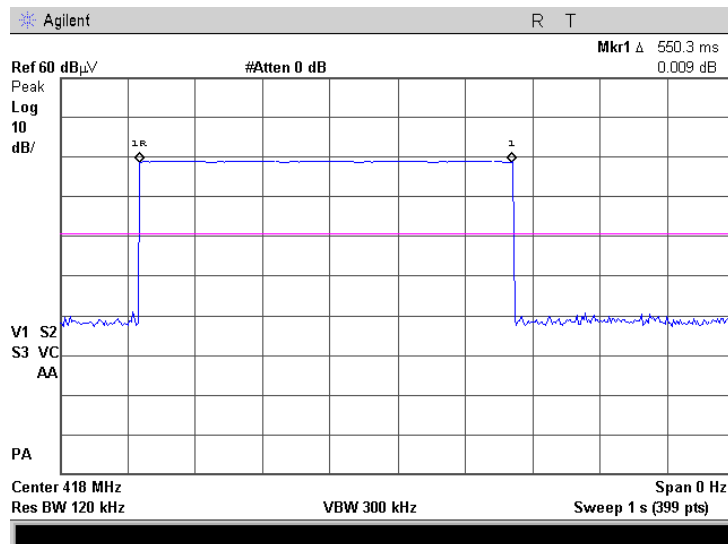
Plot 7.1.5 Polling / supervision transmission duration – one burst
