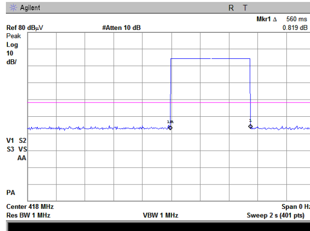
Plot 7.2.22 Transmission burst period
