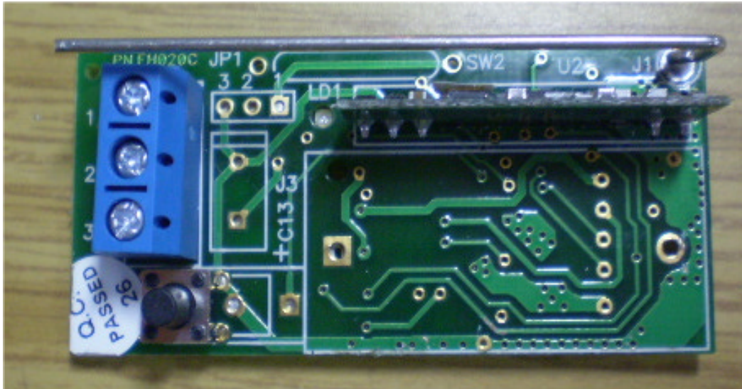
Photograph No.3 EL2606 main PCB without battery compartment
