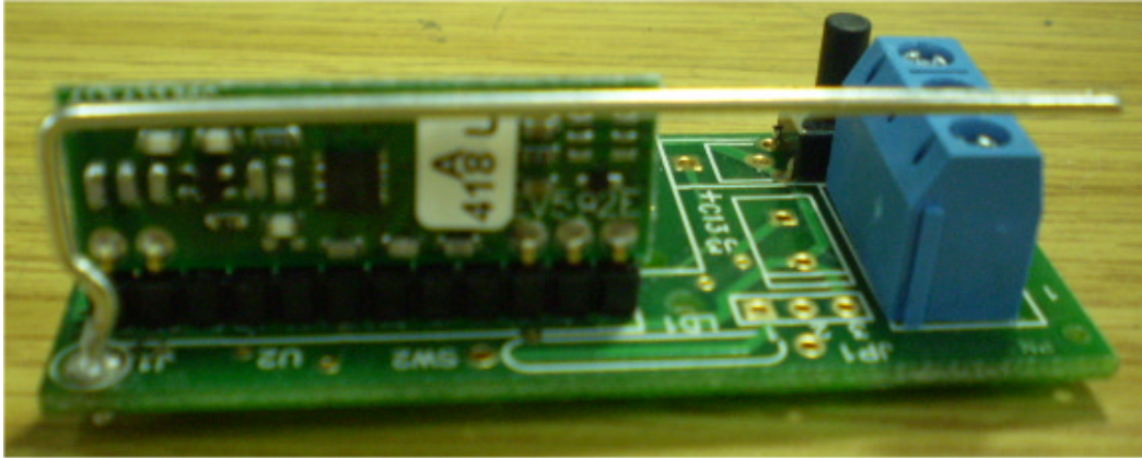
Photograph No.5 EL2606 main PCB side view with RF module and antenna
