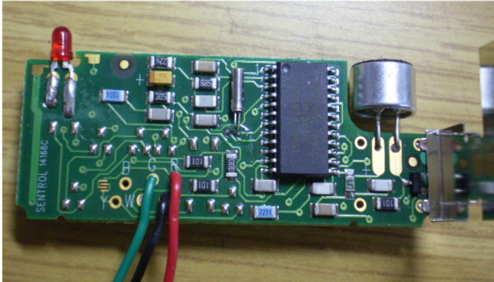
Photograph No.9 EL2606 sensor PCB front view with shield removed
