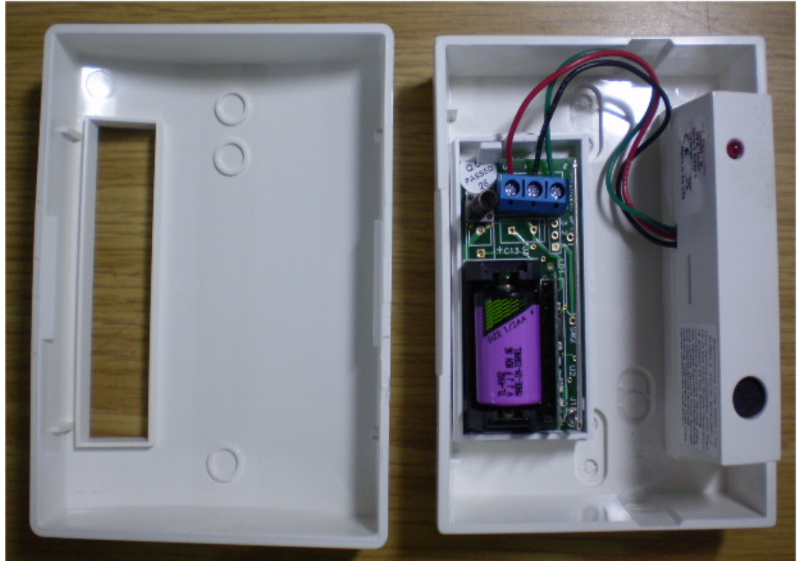
Photograph No.1 EL2606 glass break sensor internal view
