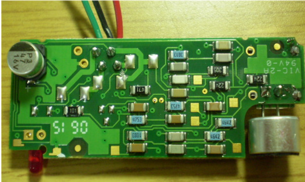
Photograph No.10 EL2606 sensor PCB second side view
