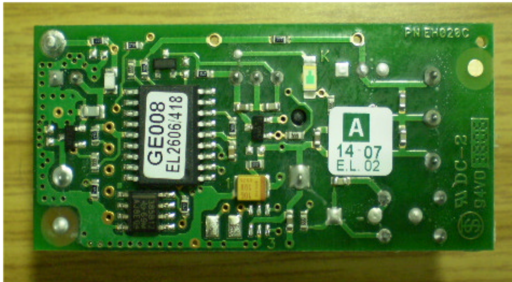
Photograph No.4 EL2606 main PCB rear side view
