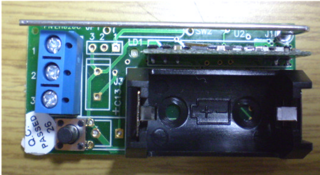
Photograph No.2 EL2606 main PCB without battery
