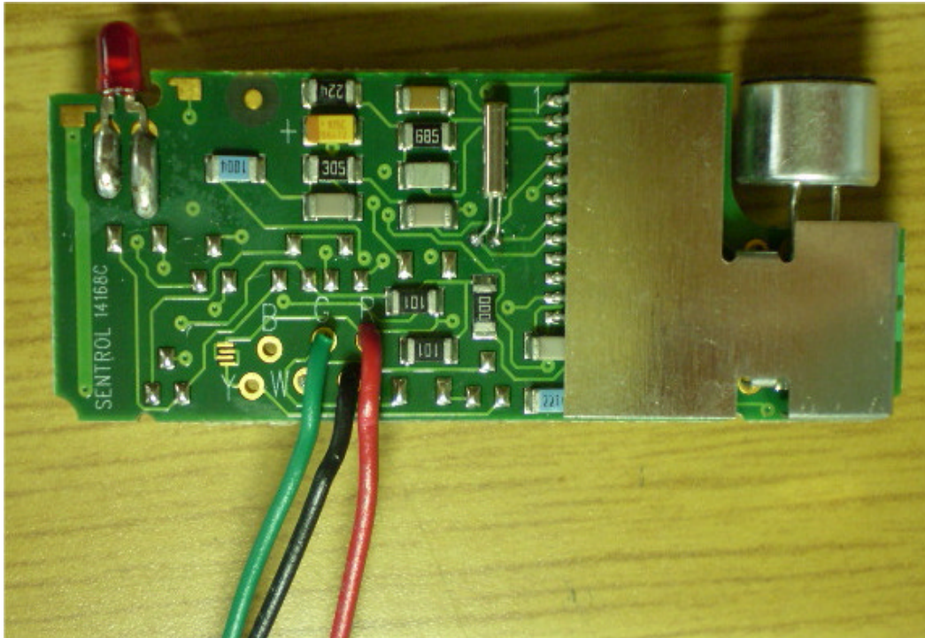
Photograph No.8 EL2606 sensor PCB front view
