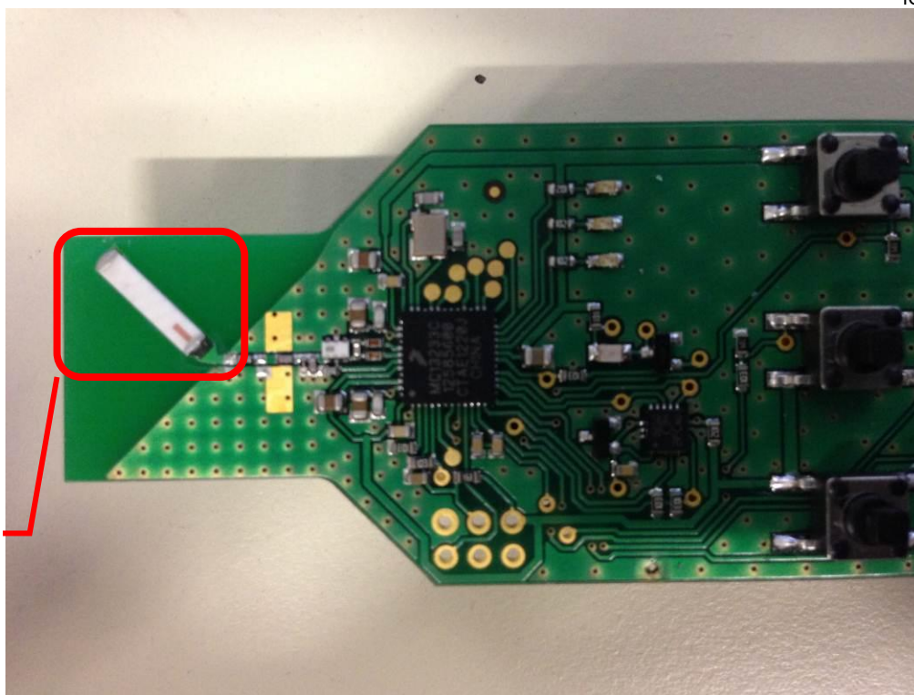
Ceramic Antenna
