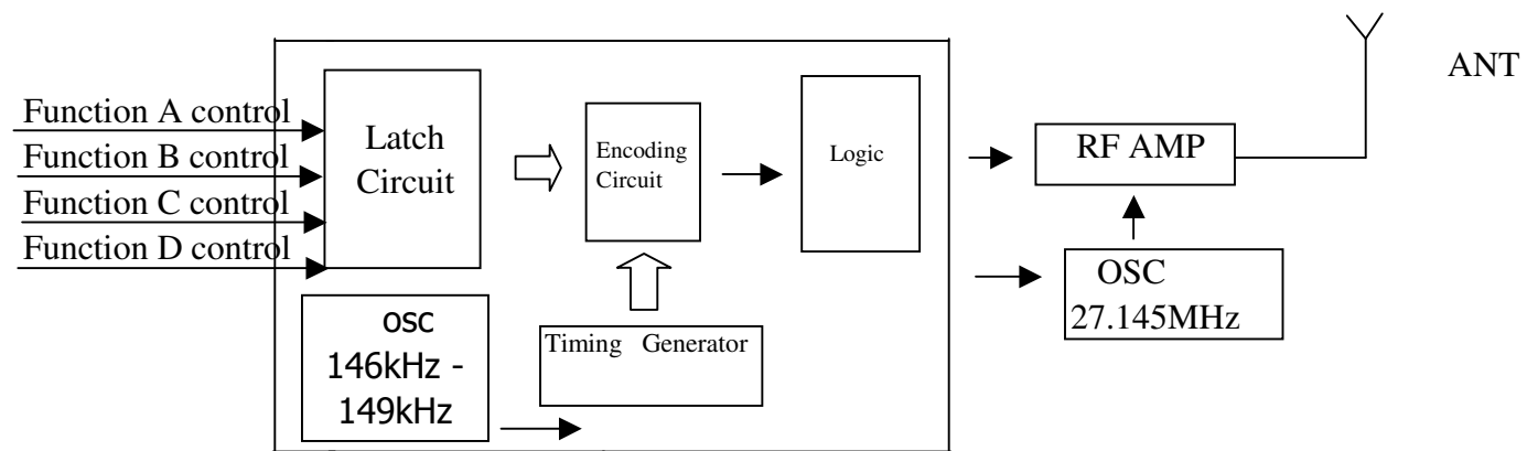
TX Block Diagram
