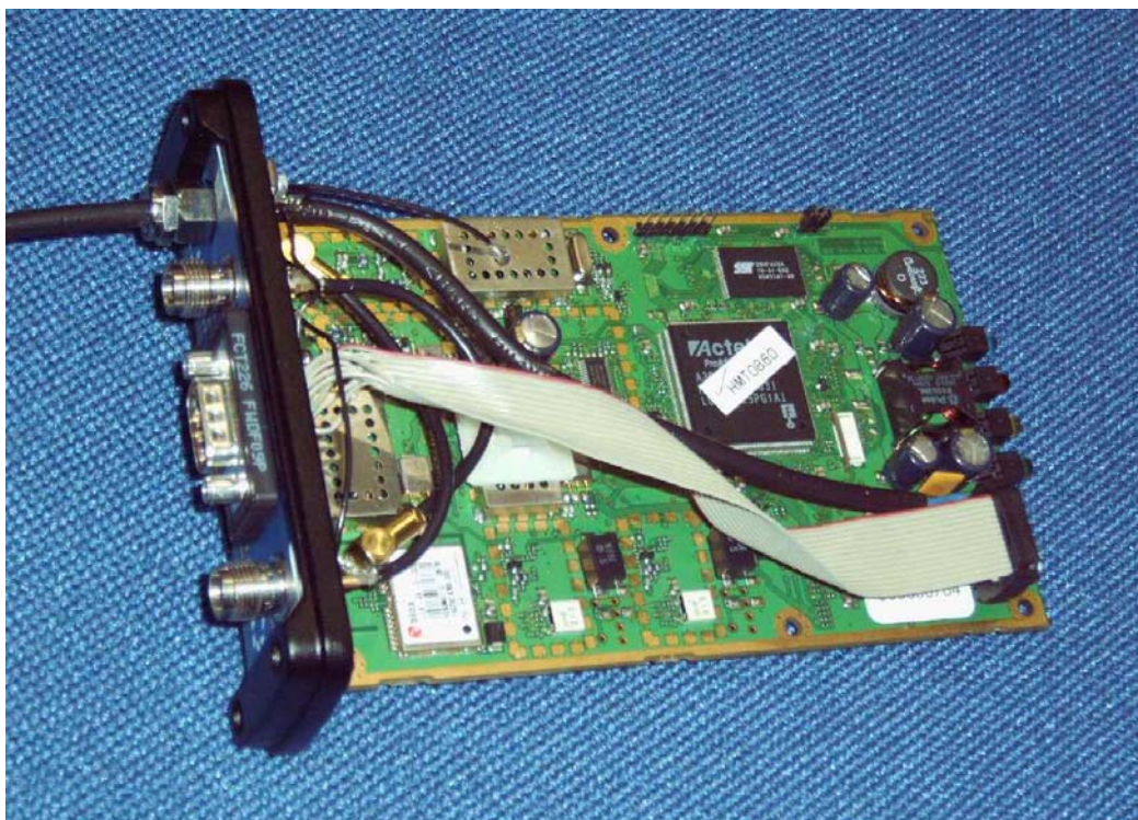
Fig 2 - Showing Topside of PCB Assembly And Rear Panel
