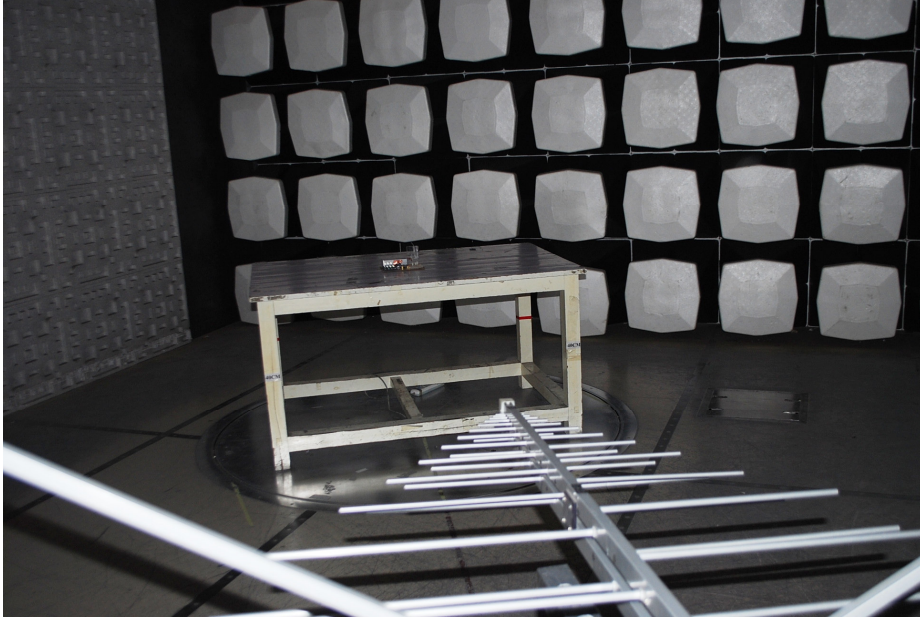
Radiated Emission
