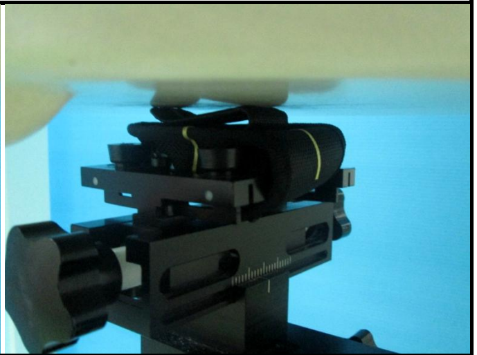
Rear Face of EUT, Holster with 0 cm Gap
