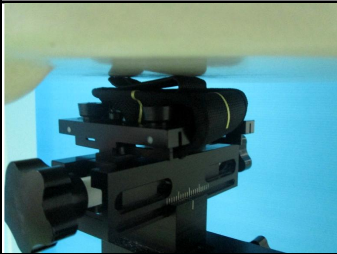
Front Face of EUT, Holster with 0 cm Gap
