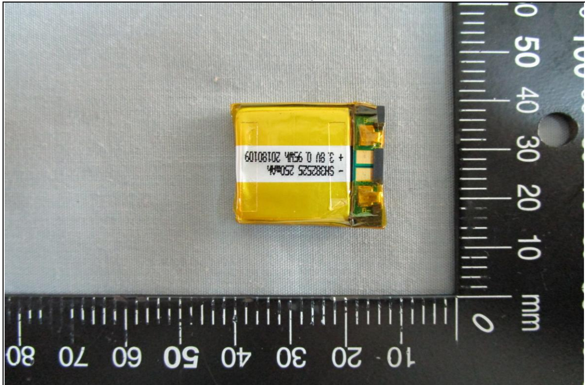
< Battery-F >
