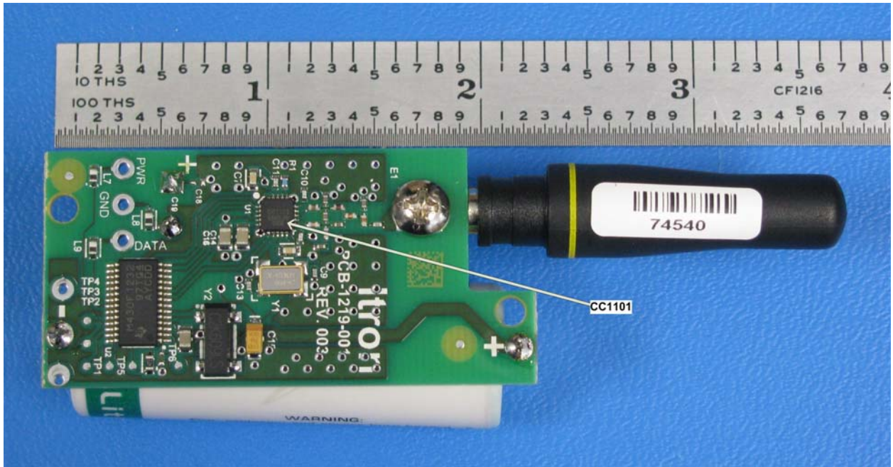
CC1101 location
