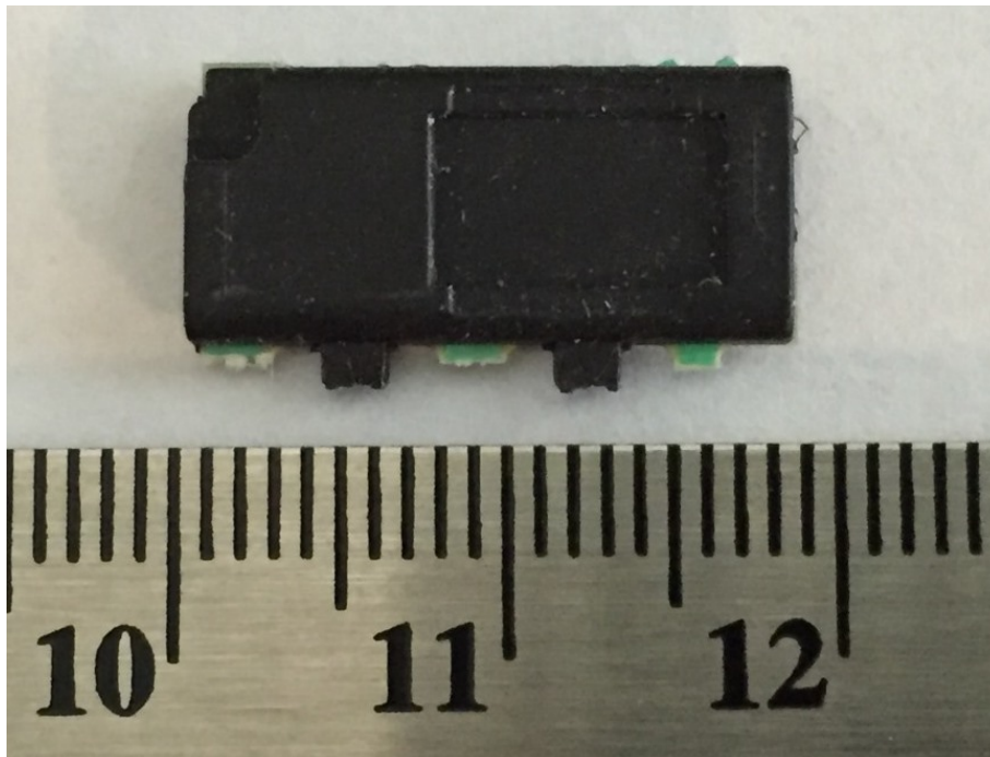
Internal PCB – Bottom View
