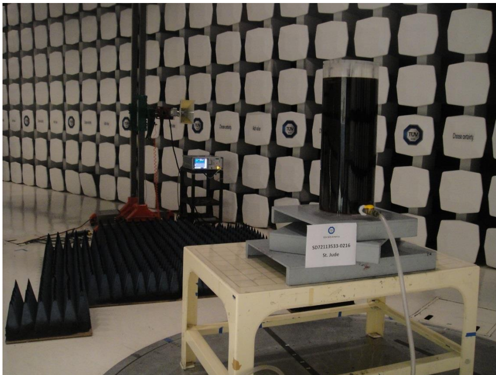
Radiated emission setup above 1GHz
