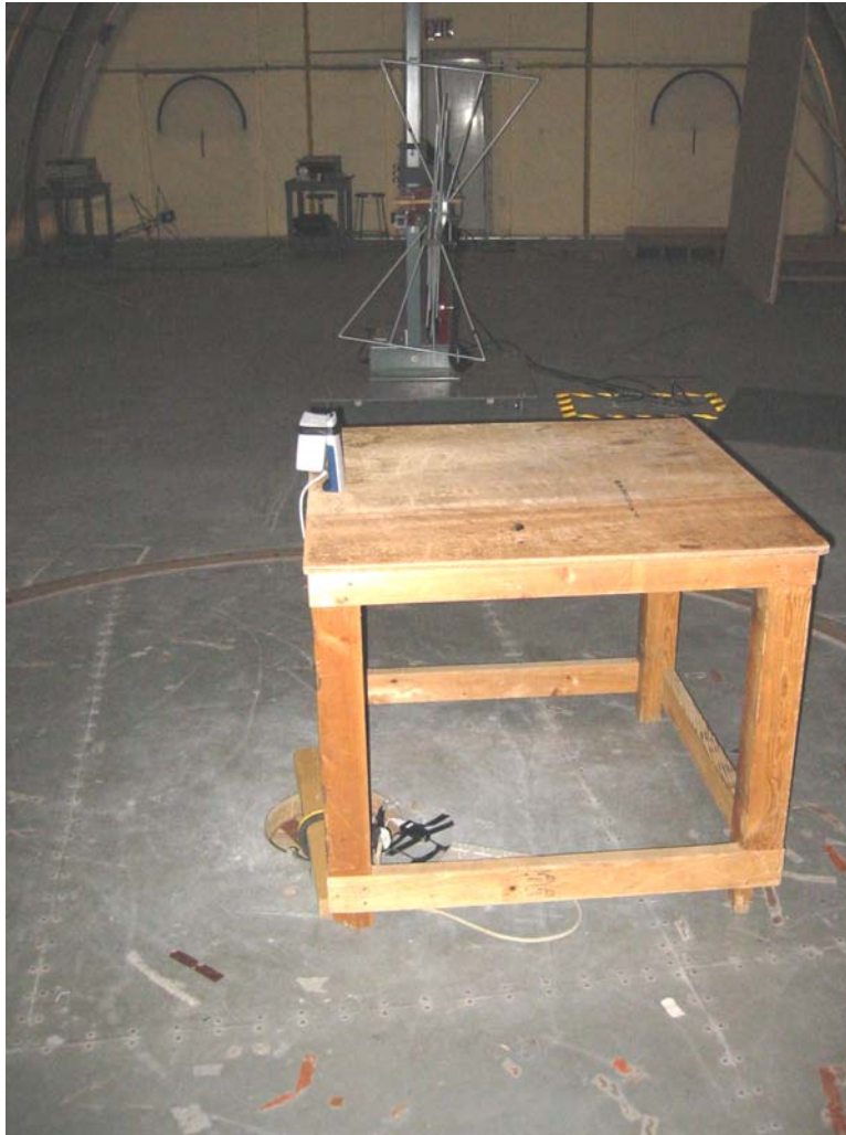
Radiated setup < 1 GHz view 2.
