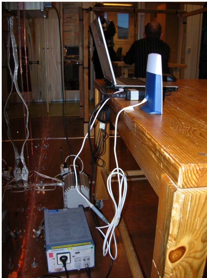
Conducted setup view 2.
