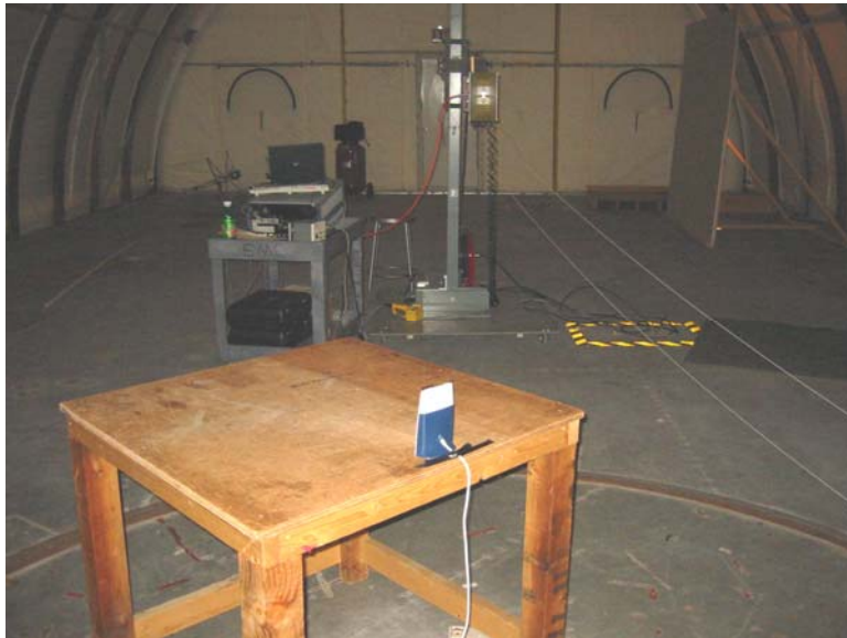
Radiated setup > 1 GHz view 2.
