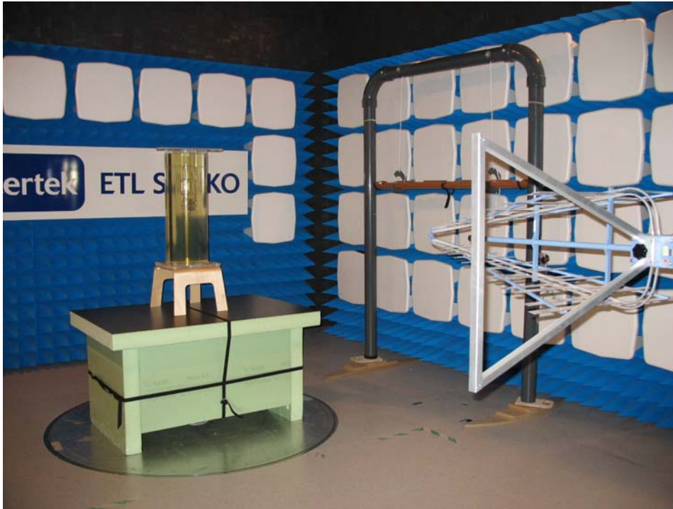
Test set-up, overview from antenna
