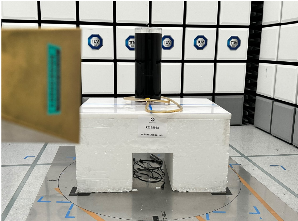
Radiated Emissions Test Setup (18GHz to 26GHz)
