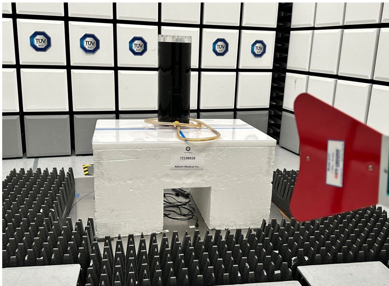
Radiated Emissions Test Setup (1GHz to 18GHz)
