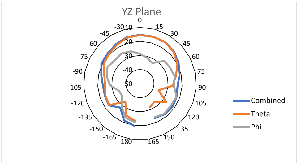
DF1 VR Header Antenna Radiation Patterns (normal orientation)
