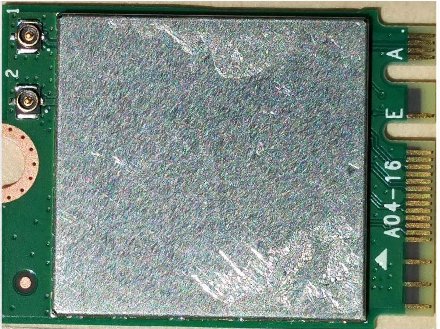
The RF Module External Photo
