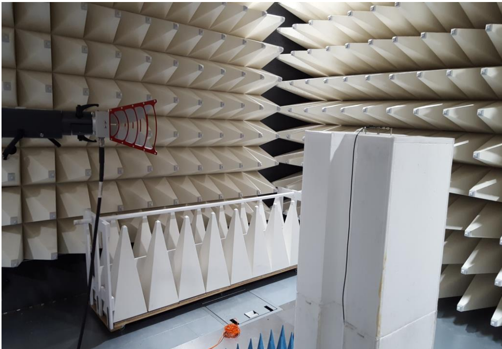
Figure C3. Radiated Setup – High Range
