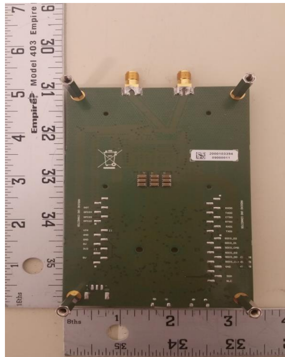
Figure C2. Conducted DUT module Rear view
