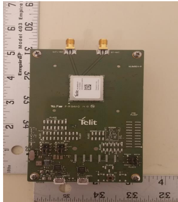
Figure C1. Conducted DUT Module top view
