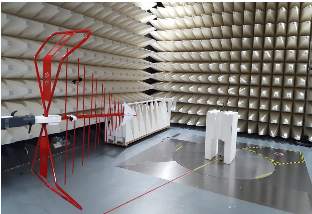
Figure C4. DUT Setup- Radiated
