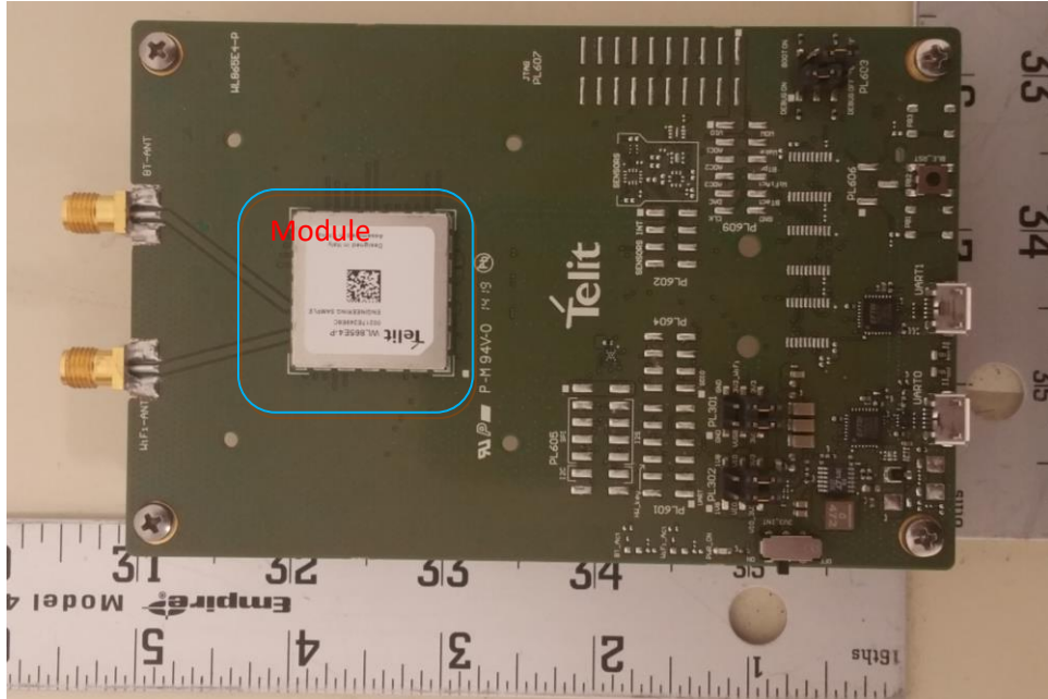
Figure B1. DUT top view
