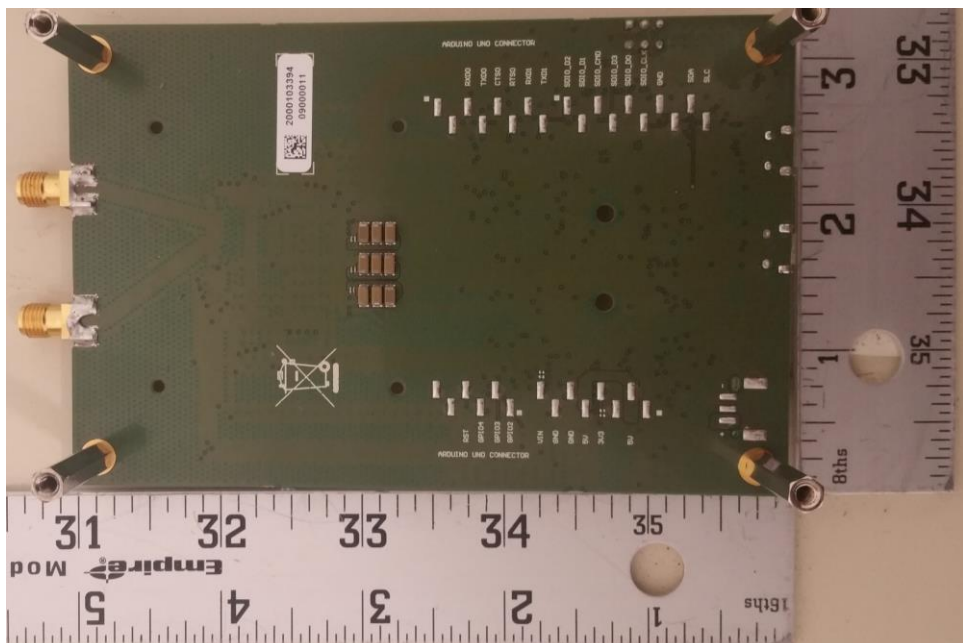
Figure B2. DUT rear view
