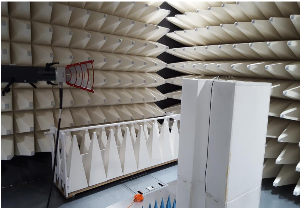
Figure B4. Radiated Setup – High Range
