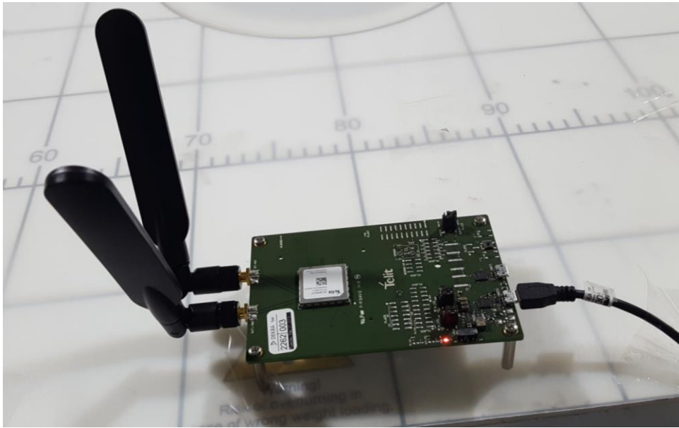
Figure B3. DUT with antennas attached
