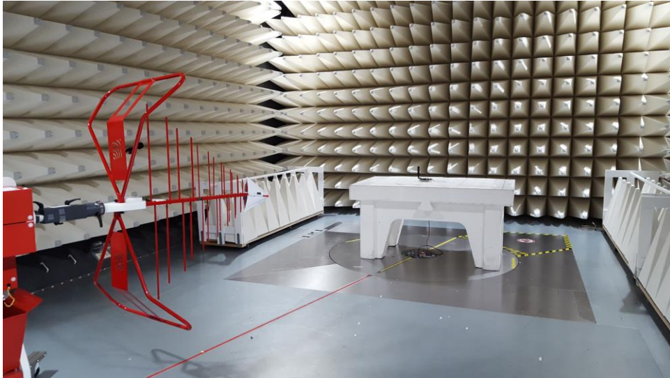
Figure B3: Low range Radiated Emission Test Setup
