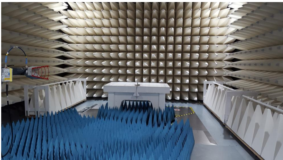
Figure B4: High range Radiated Emission Test Setup
