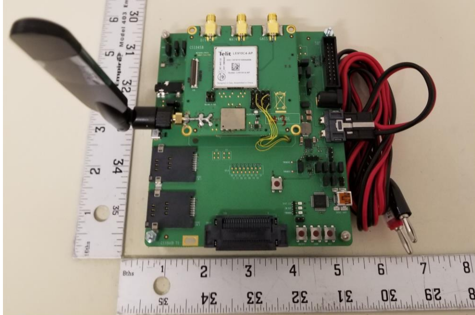
Figure B1. Top view of DUT with Cradle and antenna
