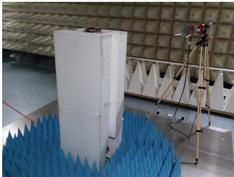
Figure C5. Radiated Setup 2
