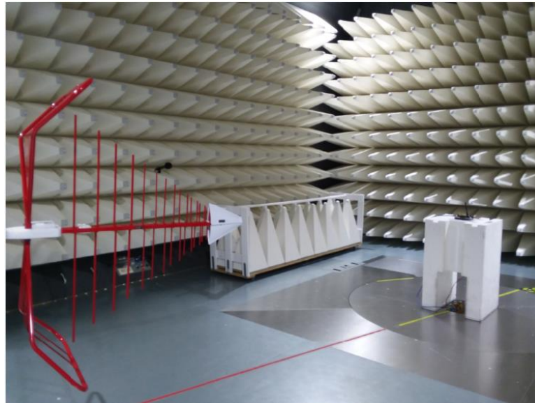
Figure C4. Radiated Setup 1
