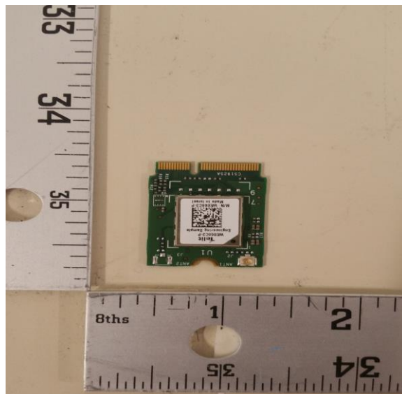
Figure C2: Conducted DUT top view with board and module
