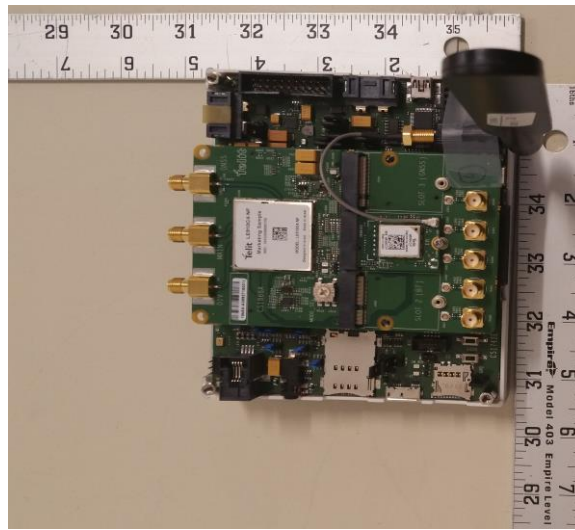
Figure C1: DUT Sample
