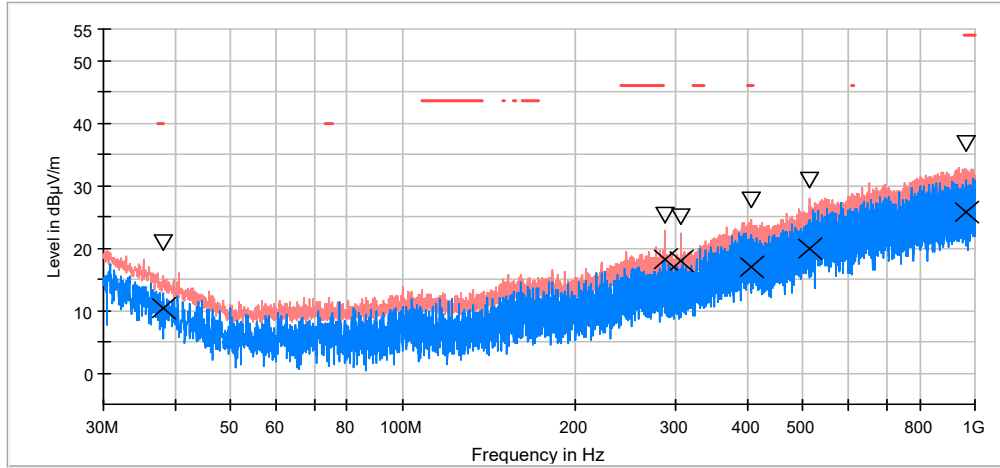
RF_FCC_15.247_E Field_30MHz_1GHz
