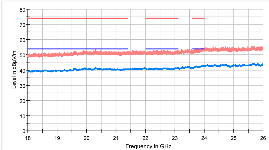
RF_FCC_15.247_E Field_18GHz_26GHz
