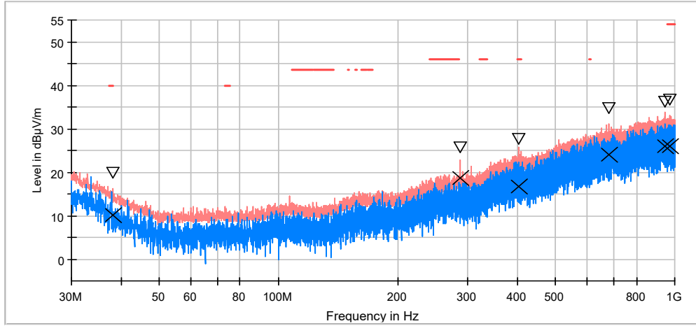
RF_FCC_15.247_E Field_30MHz_1GHz
