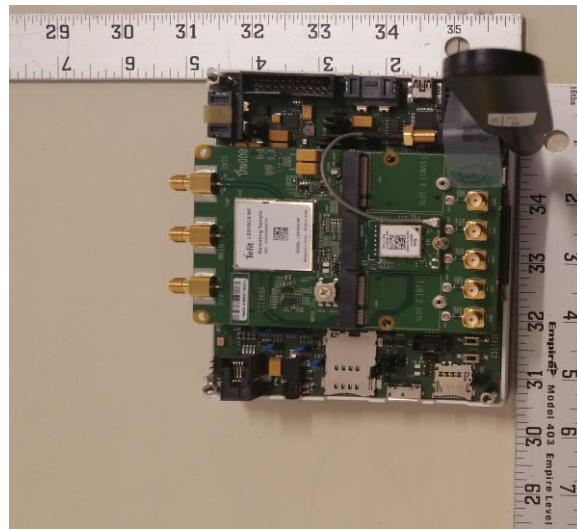
Figure D1: DUT Sample
