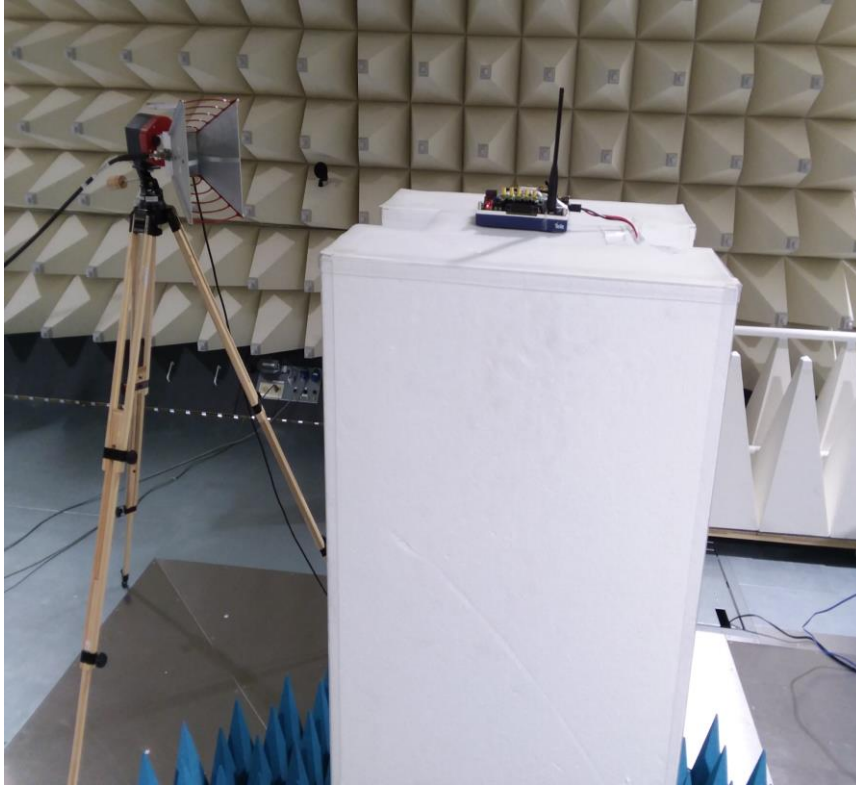
Figure D4. Radiated Setup – High Range
