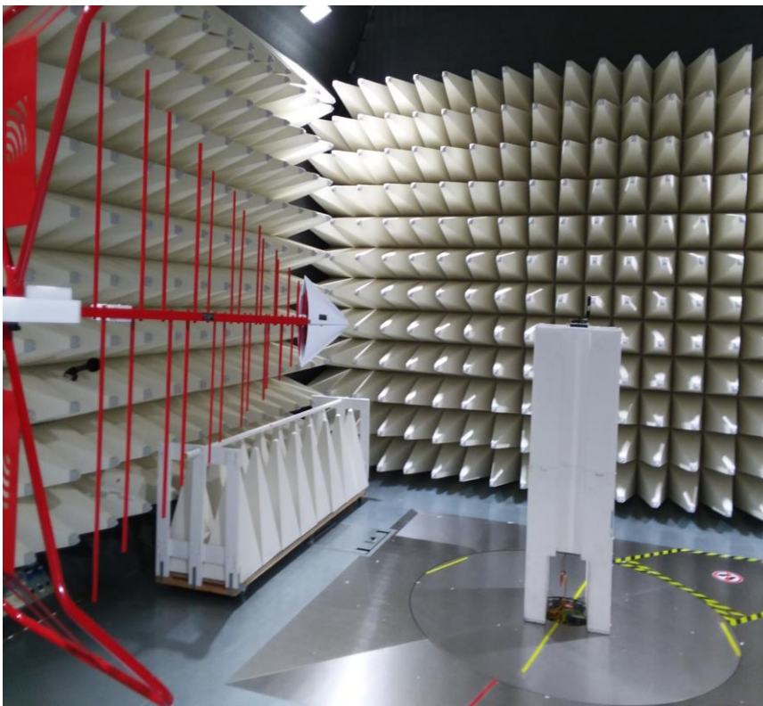
Figure D5. DUT Setup - Radiated
