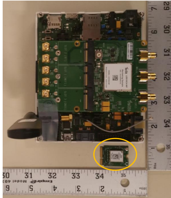
Figure B3. DUT and its cradle separated view
