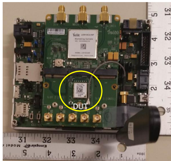
Figure B4. DUT on its cradle view
