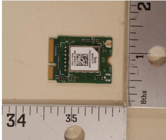
Figure B1. DUT top view
