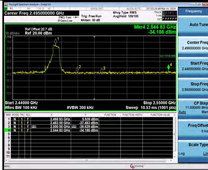
11AX20MIMO Ant2 High 2462 106Tone RU54
