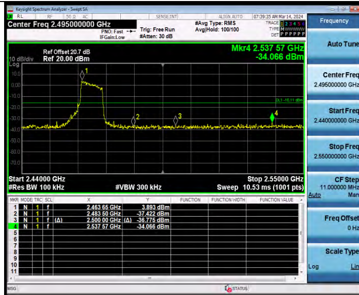
11AX20MIMO Ant2 High 2462 242Tone RU61
