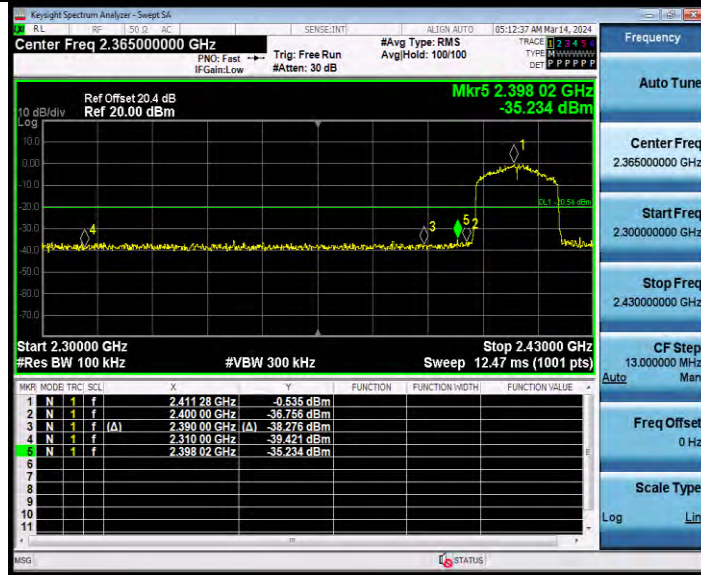
11AX20MIMO Ant2 Low 2412 26Tone RU0
