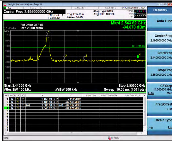
11AX20MIMO Ant2 High 2462 52Tone RU40
