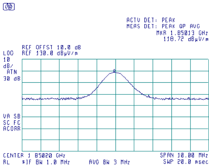
Plot 8.1.2 Transmitter carrier field strength at low frequency in horizontal antenna polarization, EUT vertical position
