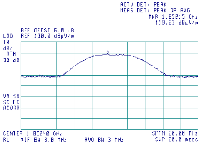
Plot 8.1.16 Transmitter carrier field strength at low frequency in horizontal antenna polarization, EUT horizontal position
