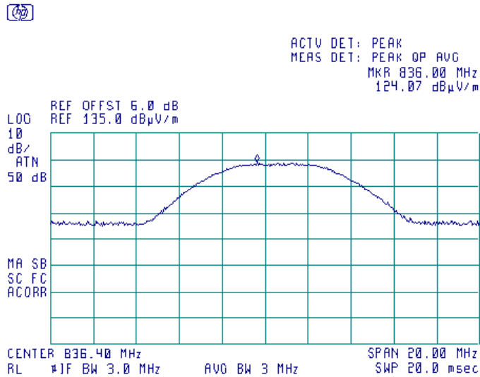
Plot 7.1.17 Transmitter carrier field strength at mid frequency in vertical antenna polarization, EUT vertical position
