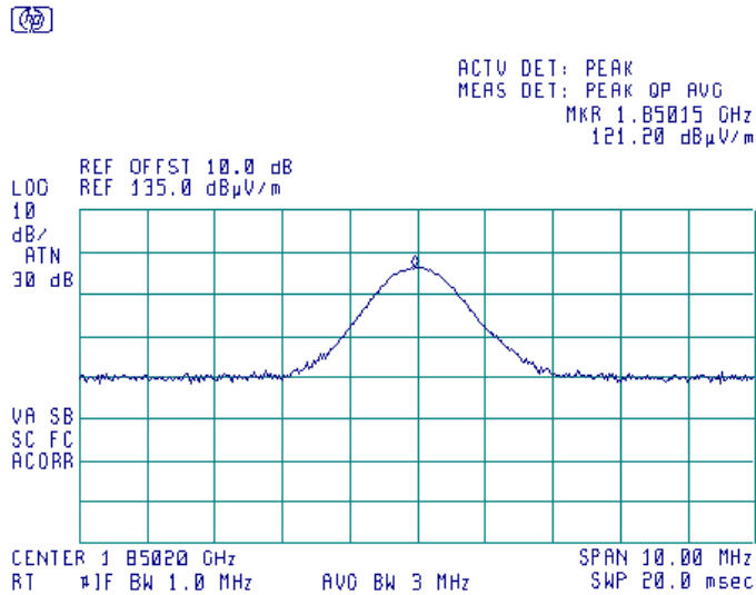
Plot 8.1.1 Transmitter carrier field strength at low frequency in vertical antenna polarization, EUT vertical position
