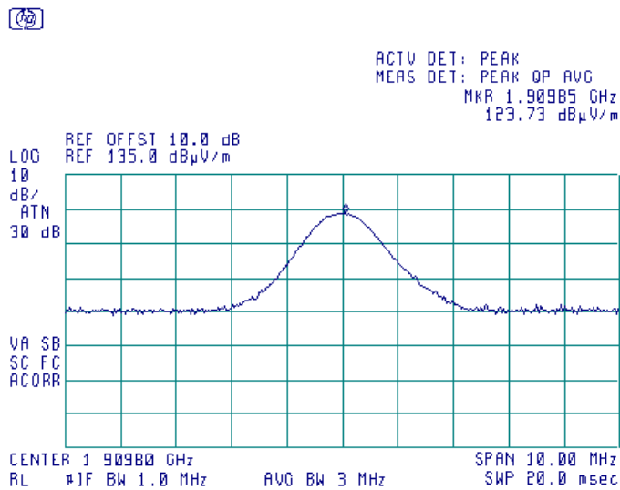
Plot 8.1.9 Transmitter carrier field strength at high frequency in vertical antenna polarization, EUT vertical position
