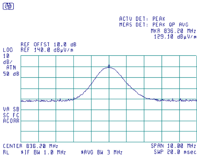
Plot 7.1.6 Transmitter carrier field strength at mid frequency in horizontal antenna polarization, EUT vertical position
