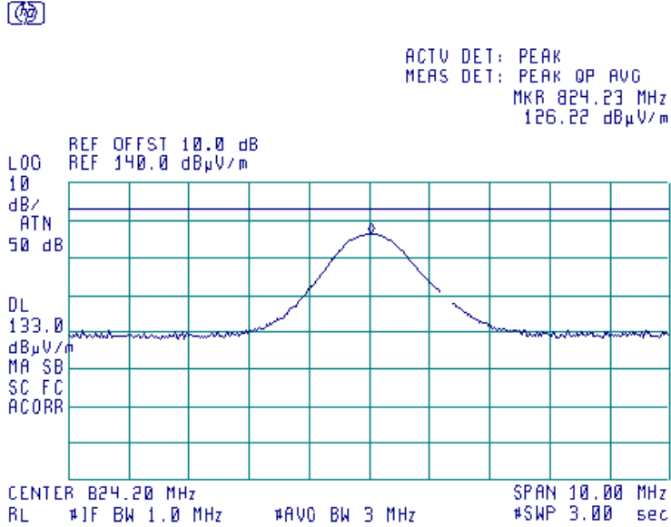
Plot 7.1.4 Transmitter carrier field strength at low frequency in horizontal antenna polarization, EUT horizontal position
