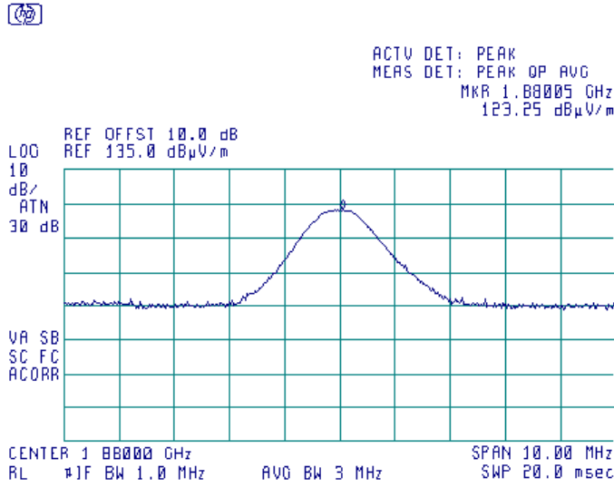
Plot 8.1.6 Transmitter carrier field strength at mid frequency in horizontal antenna polarization, EUT vertical position
