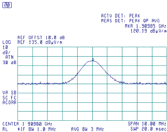
Plot 8.1.10 Transmitter carrier field strength at high frequency in horizontal antenna polarization, EUT vertical position
