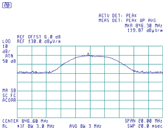
Plot 7.1.22 Transmitter carrier field strength at high frequency in horizontal antenna polarization, EUT vertical position
