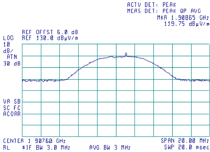
Plot 8.1.24 Transmitter carrier field strength at high frequency in horizontal antenna polarization, EUT horizontal position
