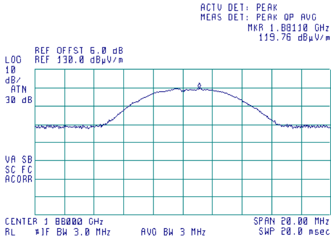
Plot 8.1.20 Transmitter carrier field strength at mid frequency in horizontal antenna polarization, EUT horizontal position
