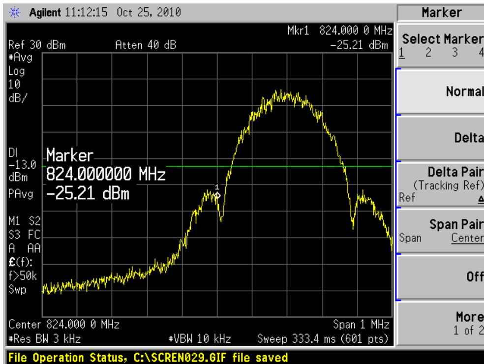
GSM 850 EGPRS 128 Channel
