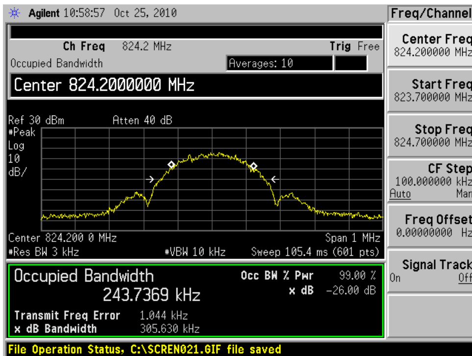
GSM 850 EGPRS CH128 Occupied Bandwidth
