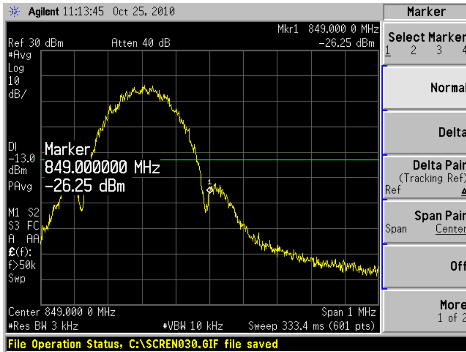
GSM 850 EGPRS 251 Channel
