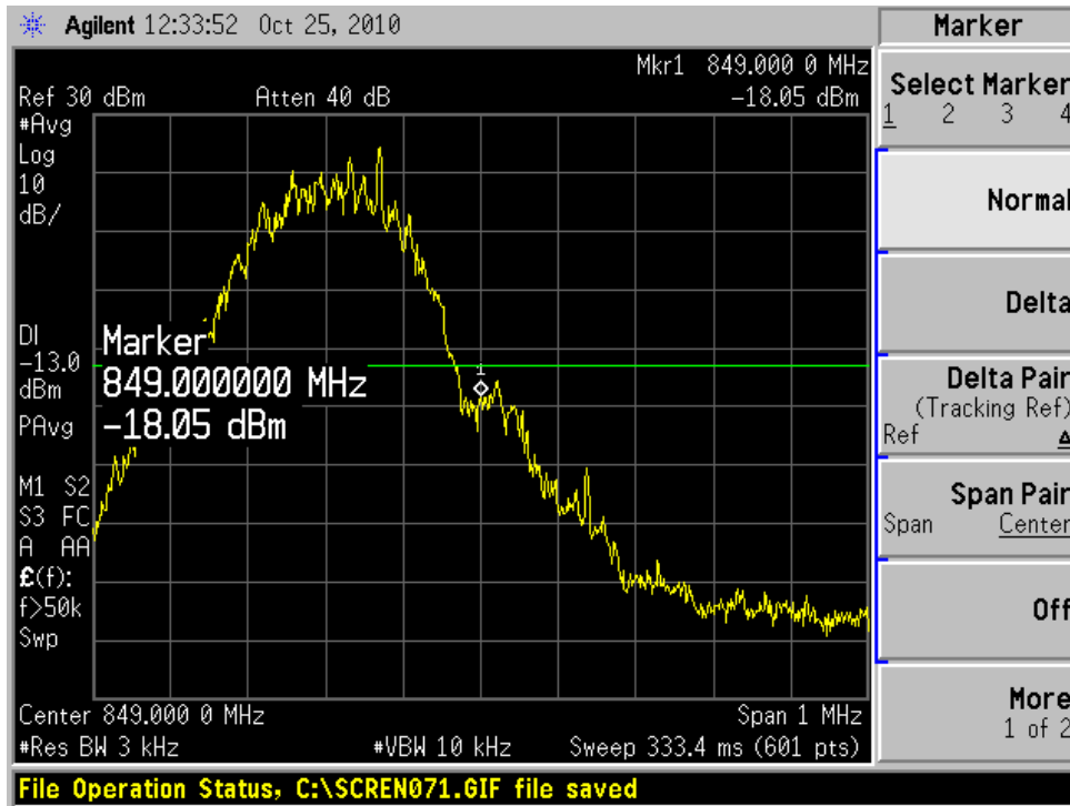
GSM 850 251 Channel
