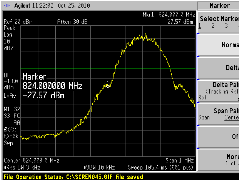
GSM 850 GPRS 128 Channel
