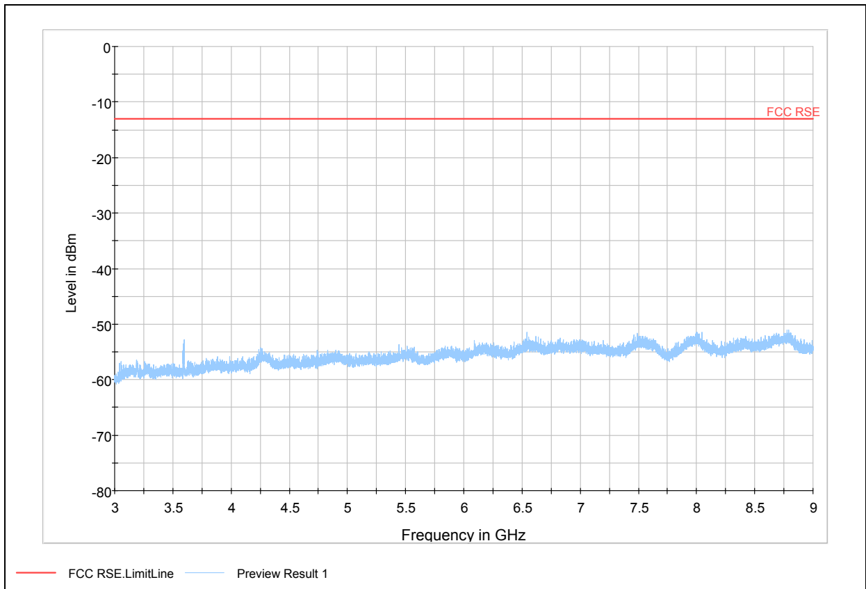
WCDMA Band V 4132 Channel 3GHz~9GHz
