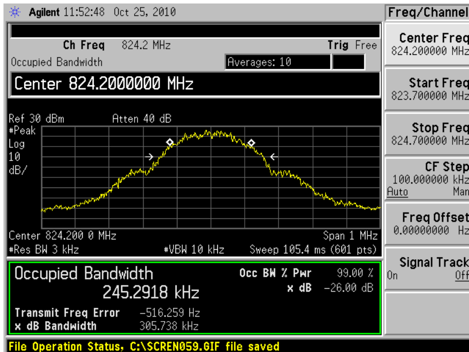
GSM 850 CH128 Occupied Bandwidth
