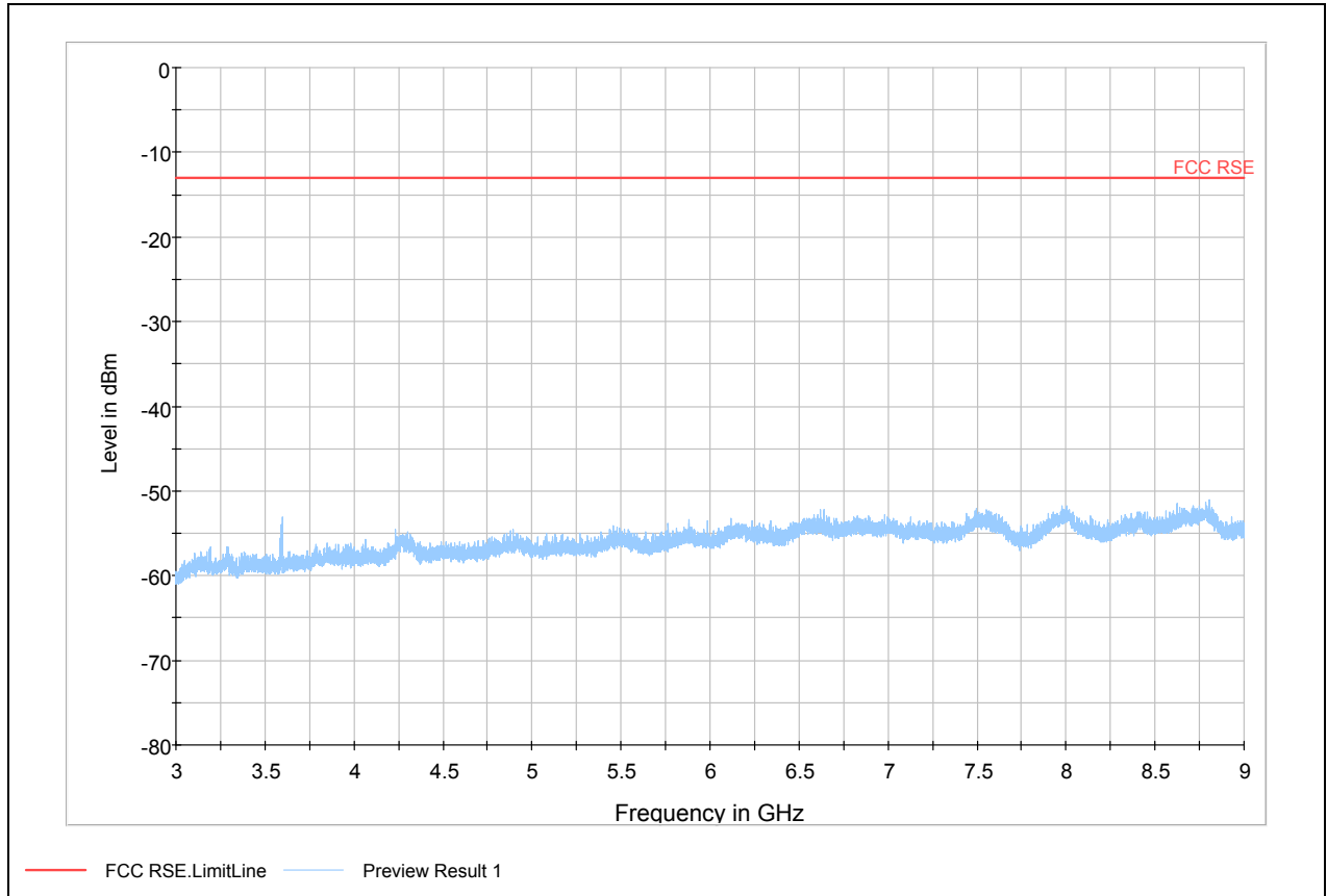
GSM 850 251 Channel 3GHz ~9GHz
