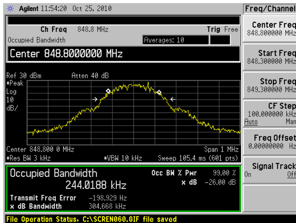
GSM 850 CH251 Occupied Bandwidth
