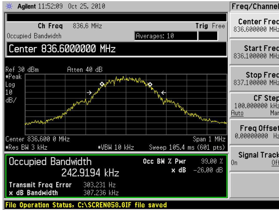
GSM 850 CH190 Occupied Bandwidth
