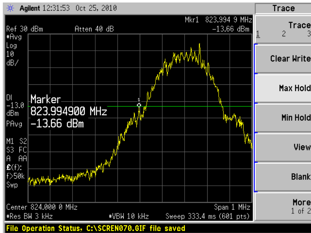
GSM 850 128 Channel
