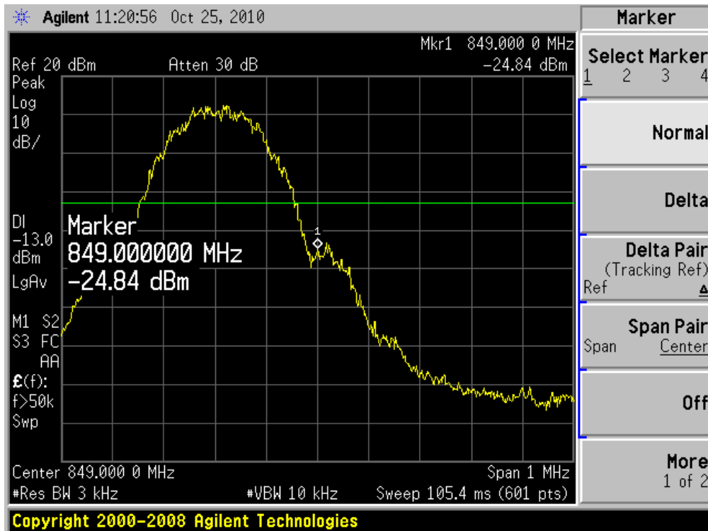
GSM 850 GPRS 251 Channel
