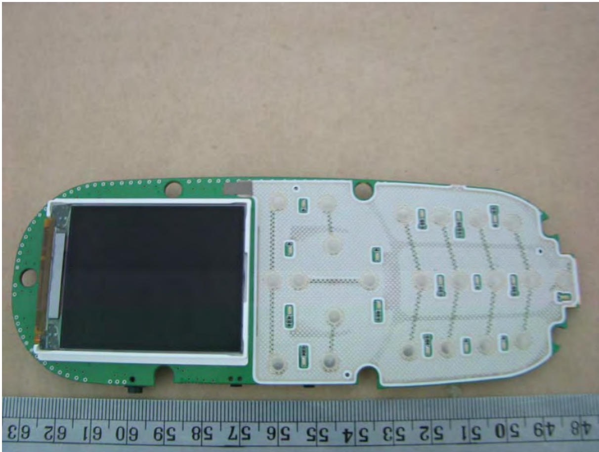
EUT Photo _ 8 of 9
