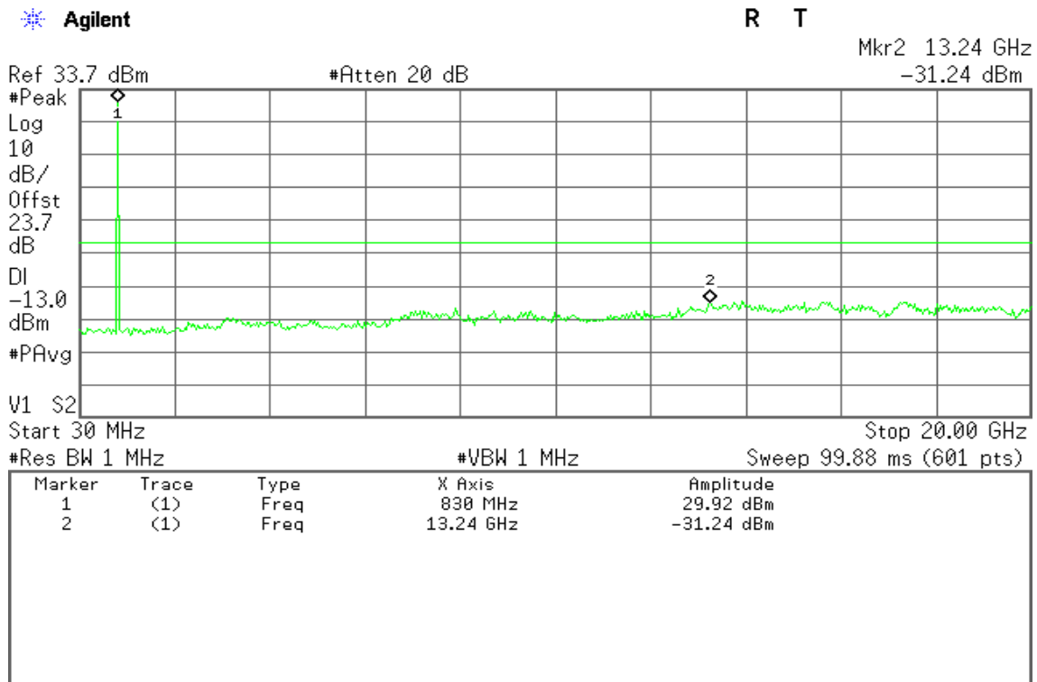
Figure 11-1: Out of Band emission at antenna terminals –EDGE CH Low
