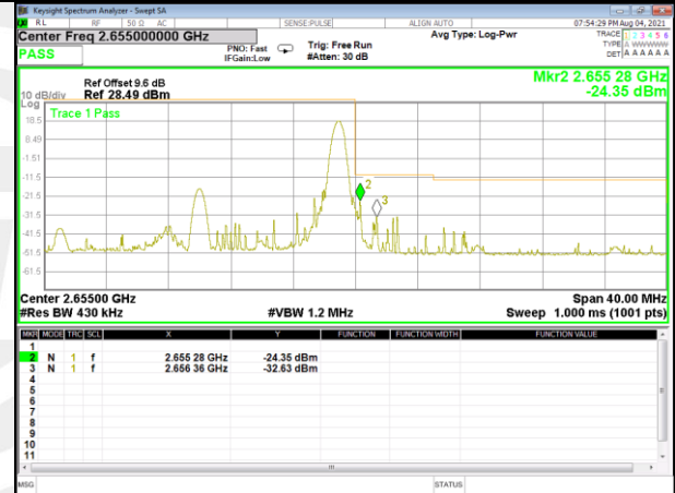
Band 41_20M_QPSK_High_Full-RB
