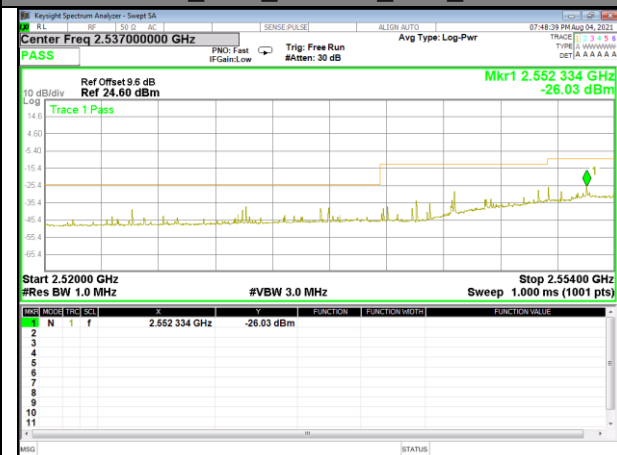
Band 41_15M_16QAM_Low_Full-RB
