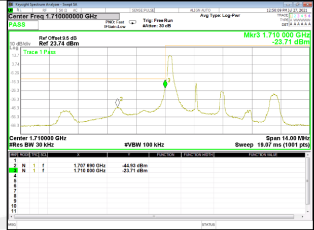
Band 66_3M_16QAM_Low_Full-RB
