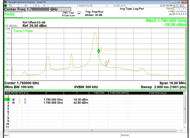
Band 66_5M_QPSK_High_Full-RB
