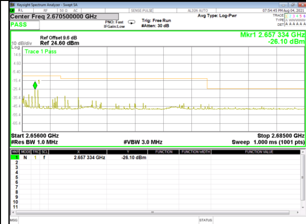
Band 41_20M_QPSK_High_Full-RB
