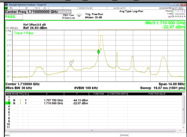
Band 66_3M_QPSK_Low_1-RB
