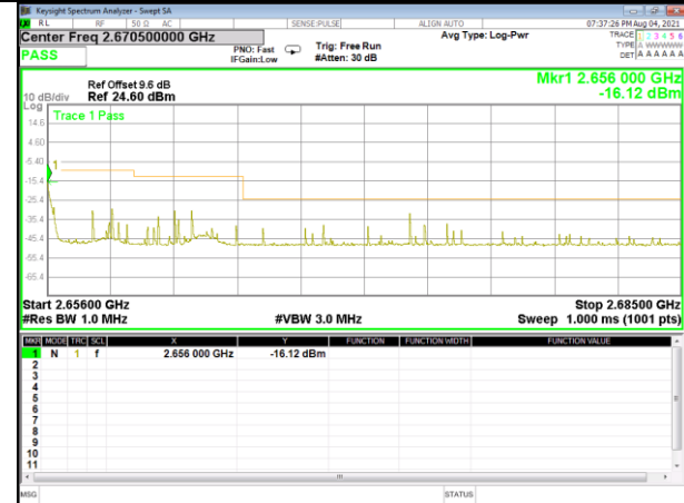
Band 41_10M_16QAM_High_Full-RB
