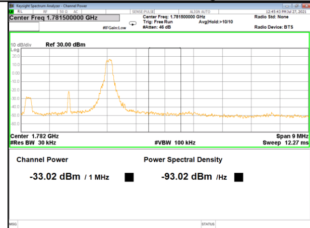
Band 66_3M_QPSK_High_Full-RB
