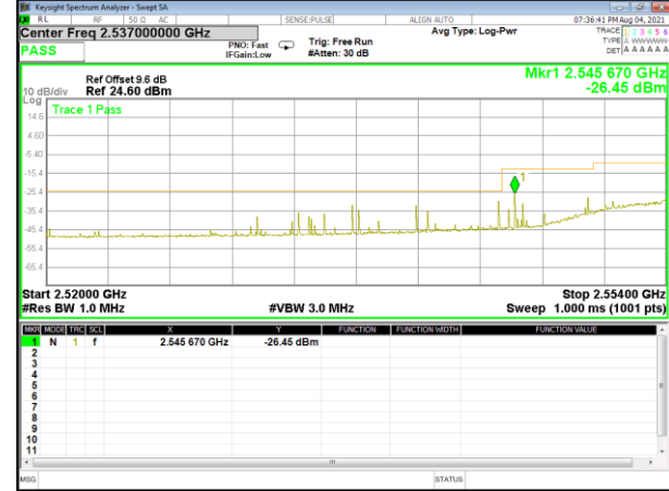
Band 41_10M_16QAM_High_1-RB
