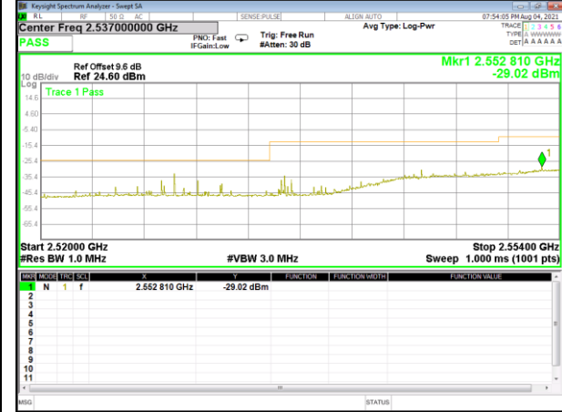
Band 41_20M_QPSK_High_1-RB
