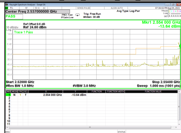
Band 41_10M_16QAM_Low_1-RB
