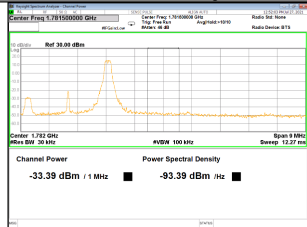
Band 66_3M_16QAM_High_1-RB
