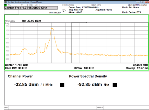
Band 66_1.4M_16QAM_High_Full-RB
