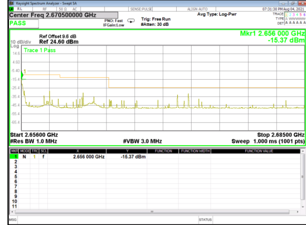
Band 41_10M_QPSK_High_Full-RB
