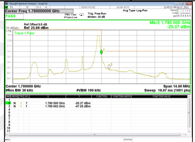
Band 66_3M_QPSK_High_Full-RB
