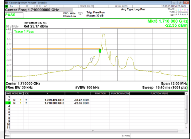
Band 66_1.4M_QPSK_Low_Full-RB
