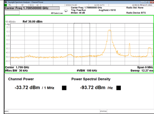
Band 66_3M_16QAM_Low_Full-RB
