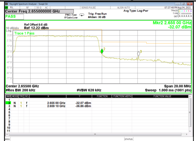
Band 41_10M_16QAM_High_Full-RB
