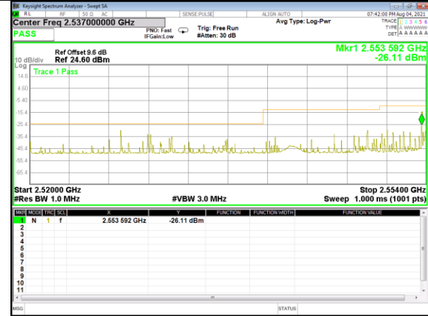
Band 41_15M_QPSK_Low_Full-RB
