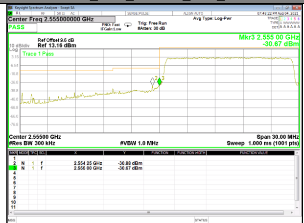
Band 41_15M_16QAM_Low_Full-RB
