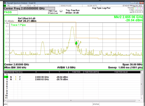
Band 41_15M_QPSK_High_1-RB
