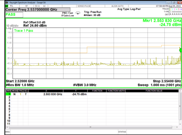
Band 41_20M_16QAM_Low_Full-RB
