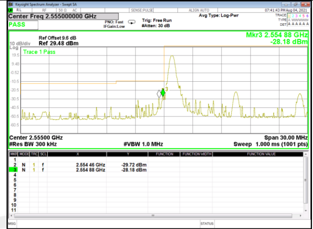
Band 41_15M_QPSK_Low_Full-RB
