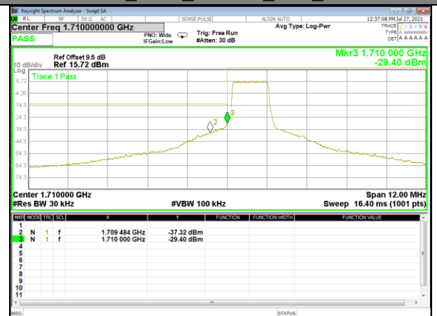
Band 66_1.4M_16QAM_Low_Full-RB
