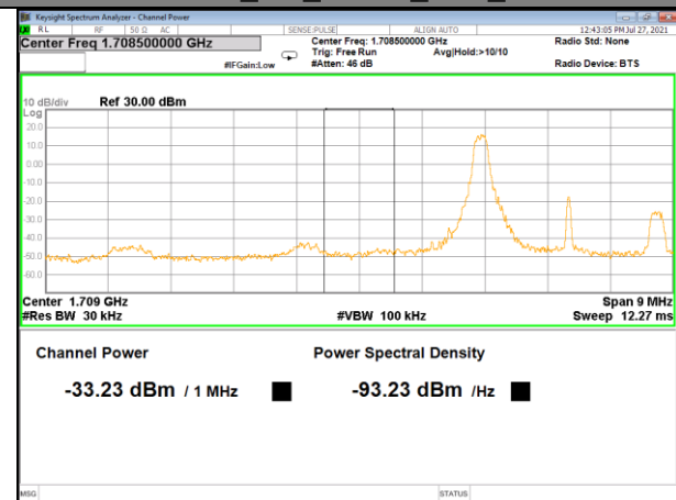
Band 66_3M_QPSK_Low_1-RB
