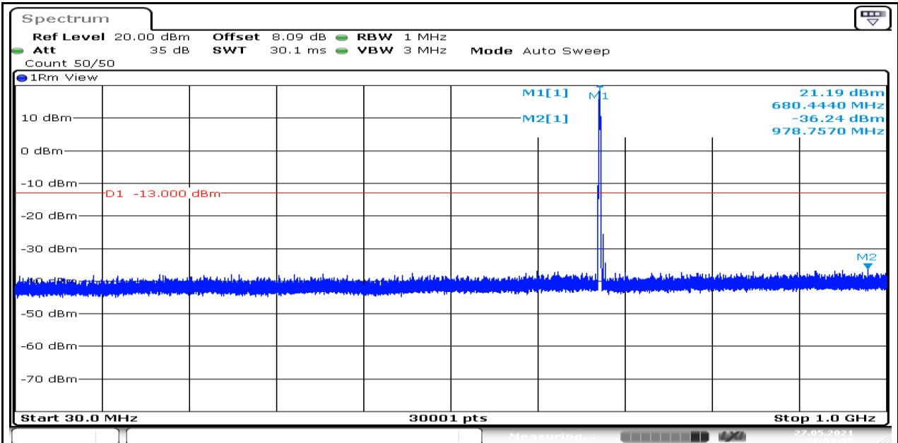
Band71-Stand-Alone-NaN-QPSK-133297-12@0-15kHz-1000-5000-1000~5000MHz@-41.58dBm--13-PASS
