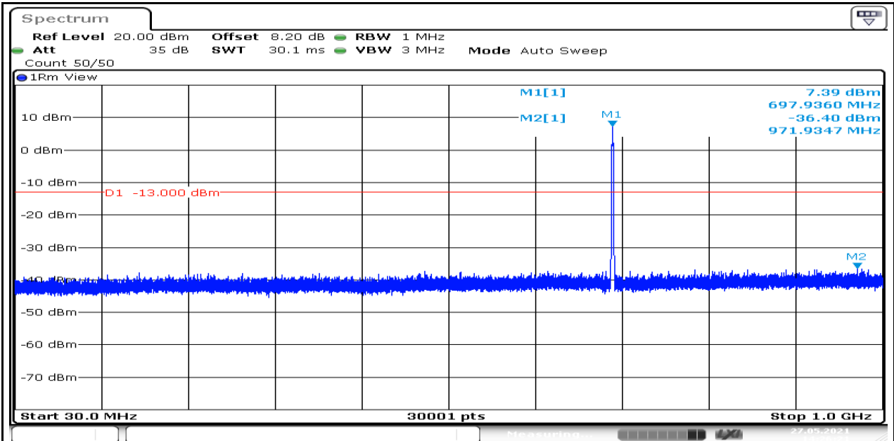
Band71-Stand-Alone-NaN-BPSK-133471-1@11-15kHz-1000-5000-1000~5000MHz@-41.56dBm--13-PASS
