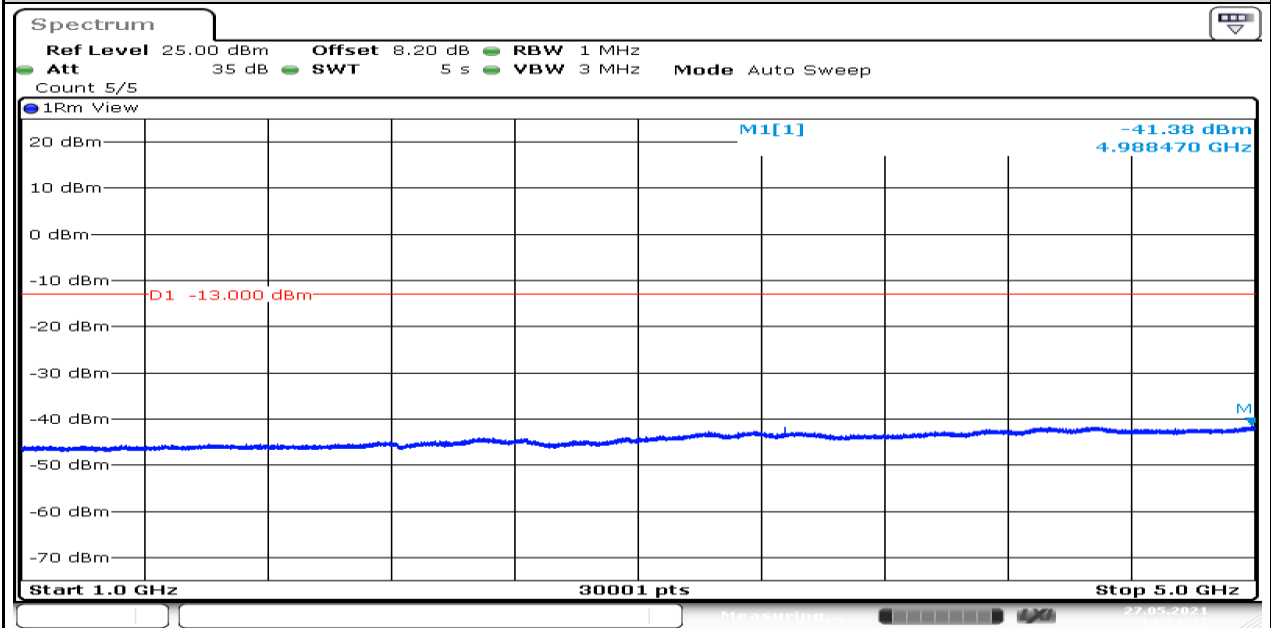
Band71-Stand-Alone-NaN-BPSK-133471-1@0-15kHz-1000-5000-1000~5000MHz@-41.38dBm-13-PASS
