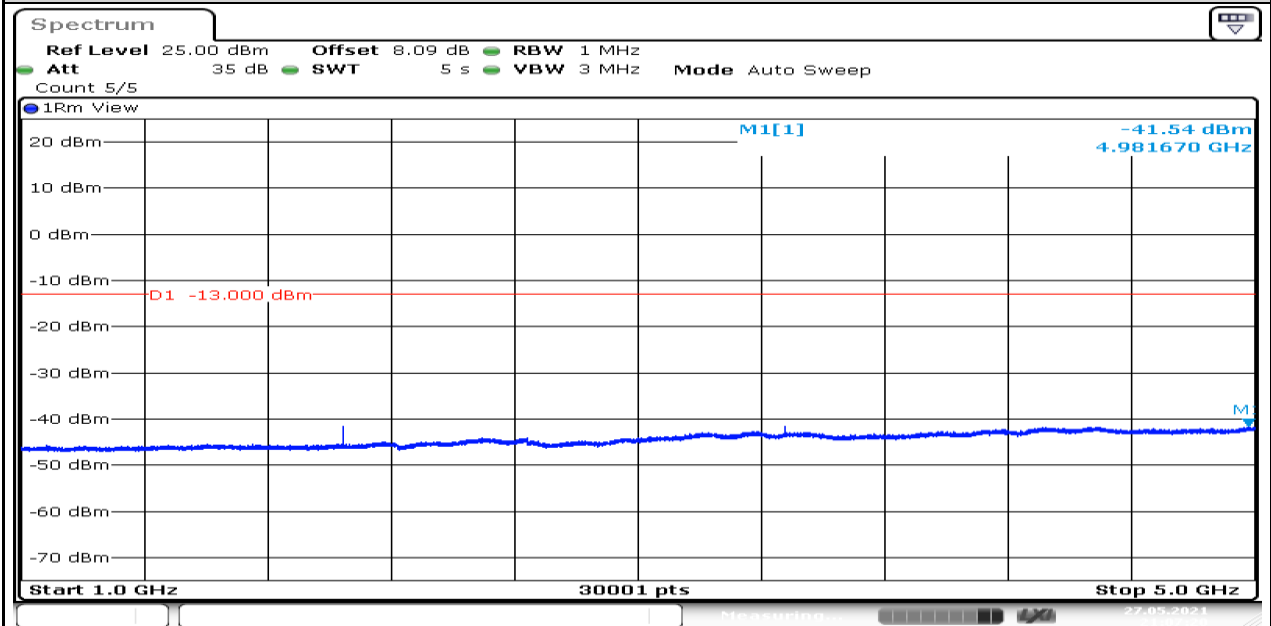
Band71-Stand-Alone-NaN-BPSK-133297-1@11-15kHz-1000-5000-1000~5000MHz@-41.54dBm--13-PASS
