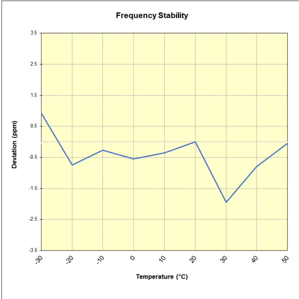
Plot 7-32. LTE Band 8 CAT-M1 Frequency Stability Chart
