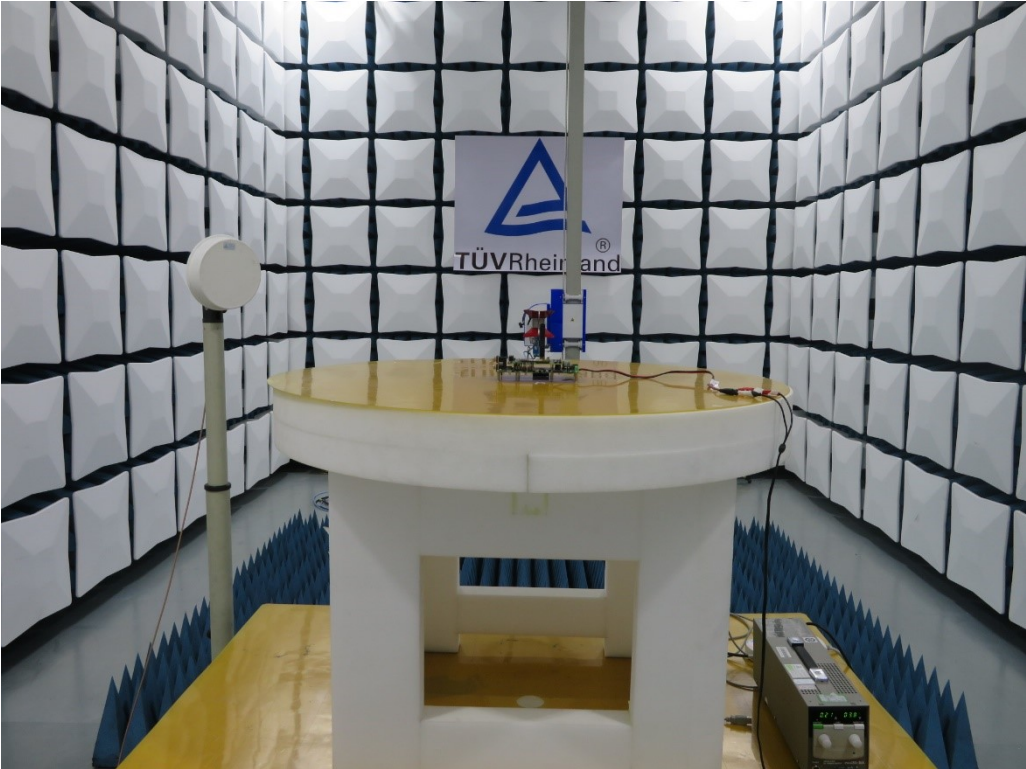
Photo 2: Radiated spurious emission for Below 1GHz
