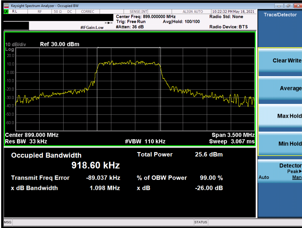
Plot 7-8. Occupied Bandwidth Plot (1.4MHz, 16-QAM, RB 5, RB Offset 0, NB=0)
