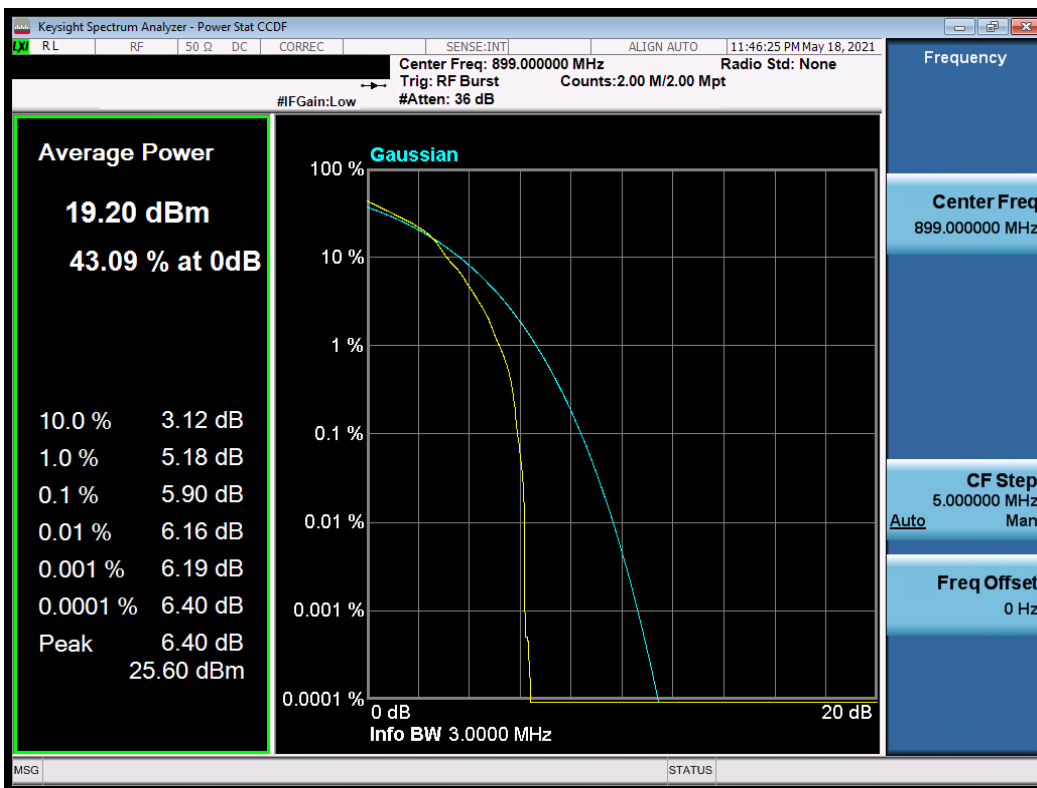
Plot 7-25. Peak to Average Ratio (3MHz, 16-QAM, RB 5, RB Offset 0, NB=1)
