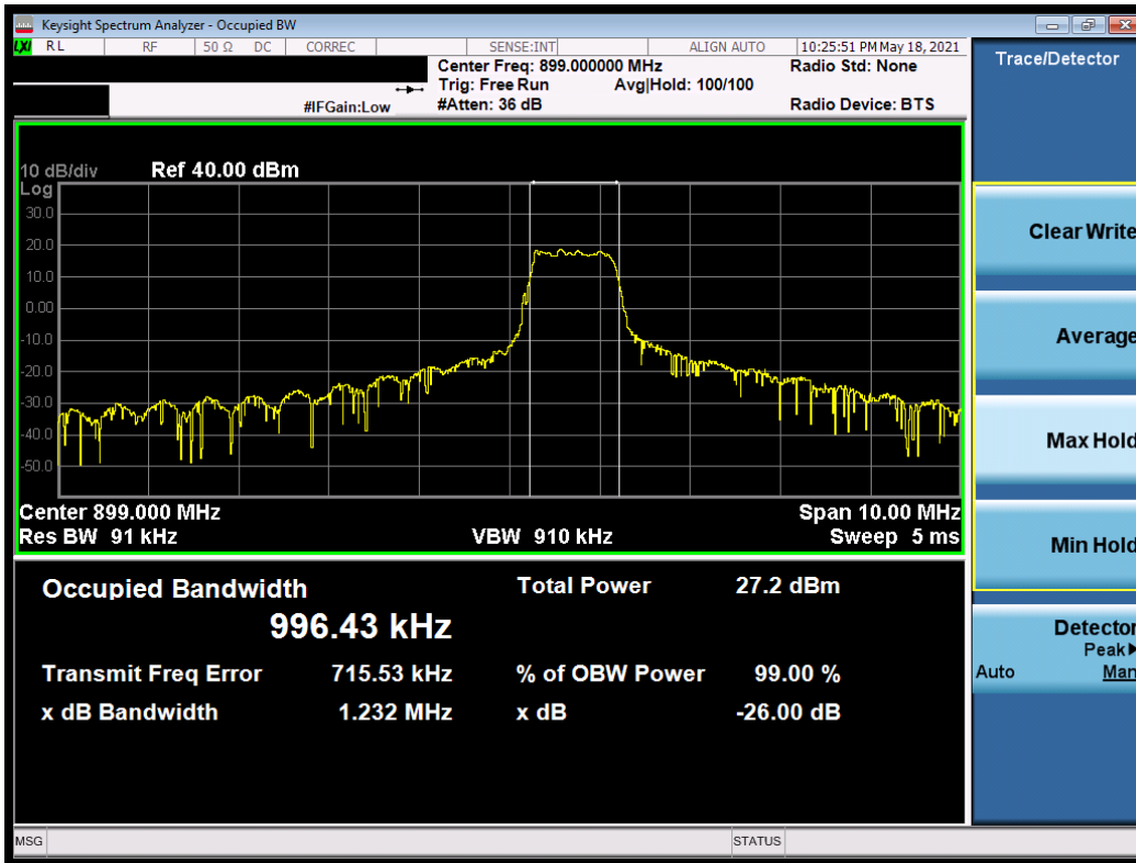
Plot 7-6. Occupied Bandwidth Plot (3MHz, 16-QAM, RB 5, RB Offset 1, NB=1)
