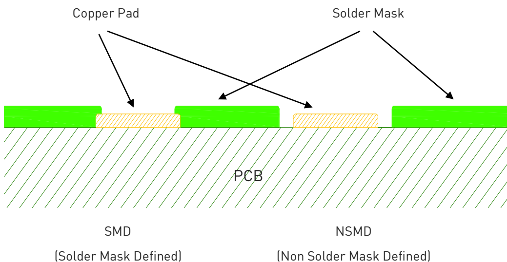
Figure 28: PCB solder pad recommendations 1W0301593 Rev.7
