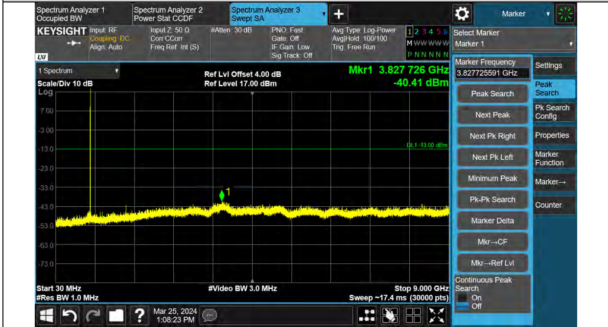
Band26-QPSK-15KHz-26788-12RB#0
