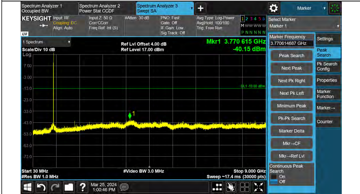
Band26-BPSK-15KHz-26788-1RB#0
