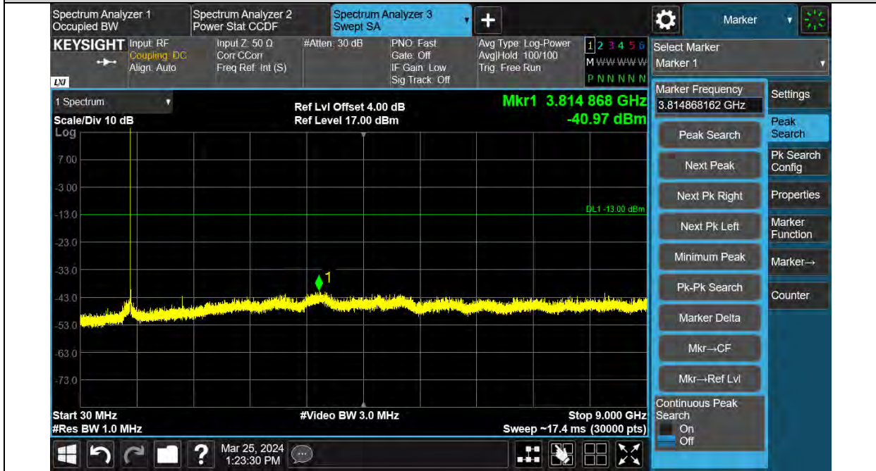
Band26-QPSK-15KHz-26692-12RB#0
