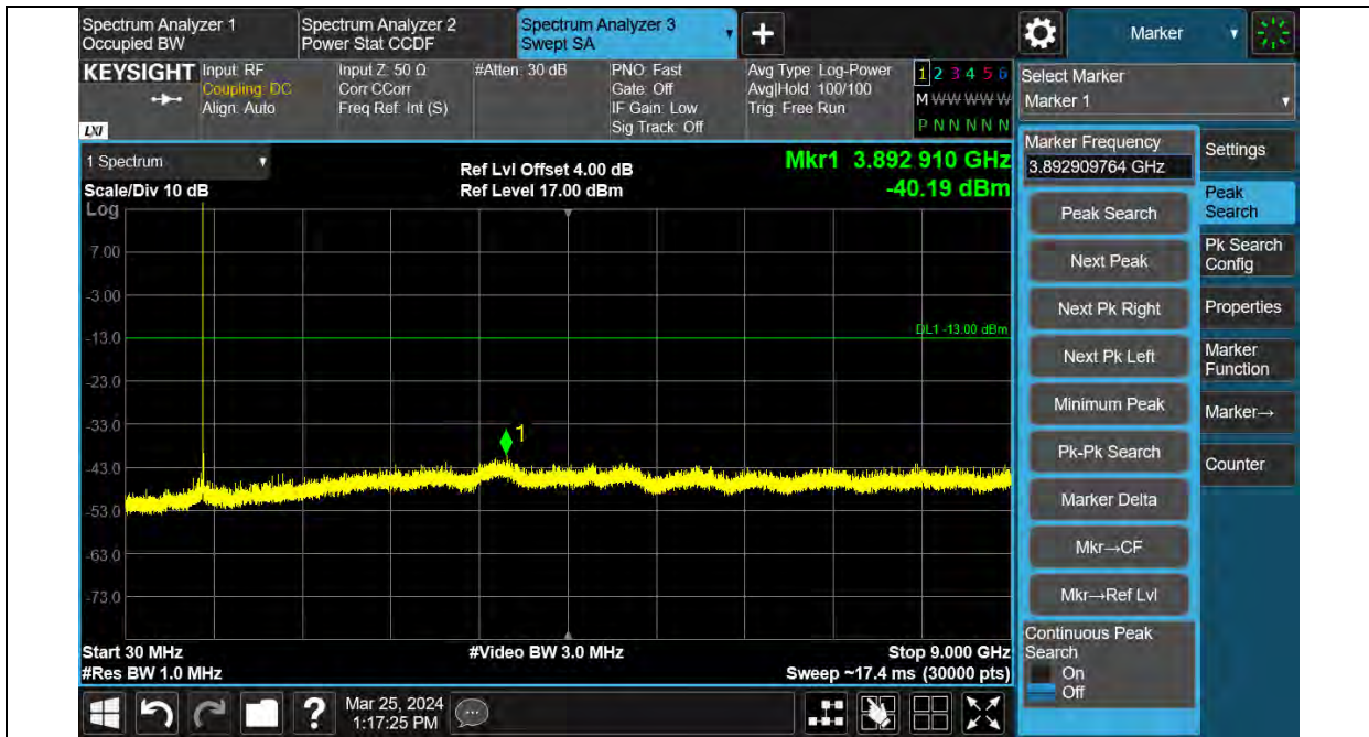
Band26-QPSK-15KHz-26740-12RB#0
