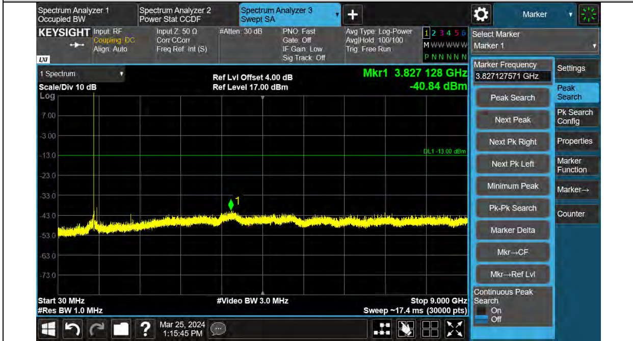
Band26-QPSK-15KHz-26740-1RB#0
