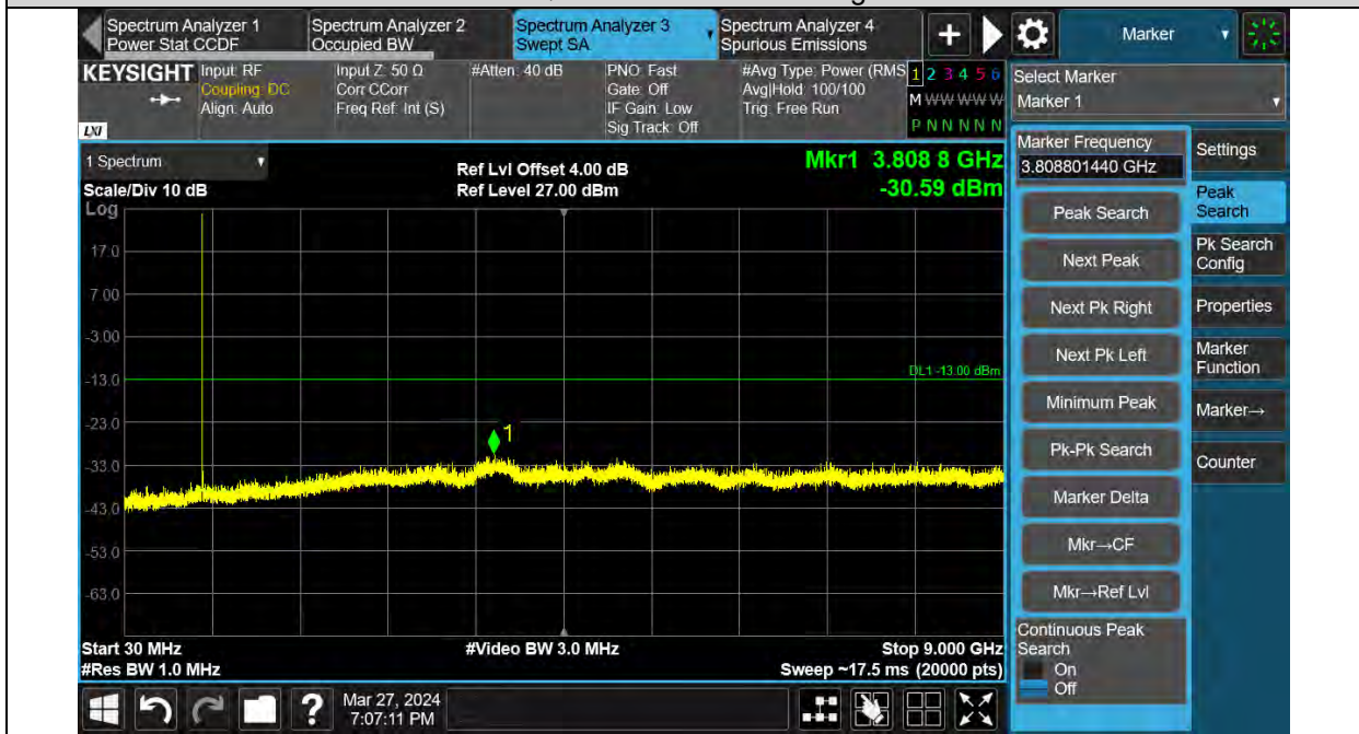
Band26-5MHz-QPSK-26715-1RB#0Range:30~9000MHz
