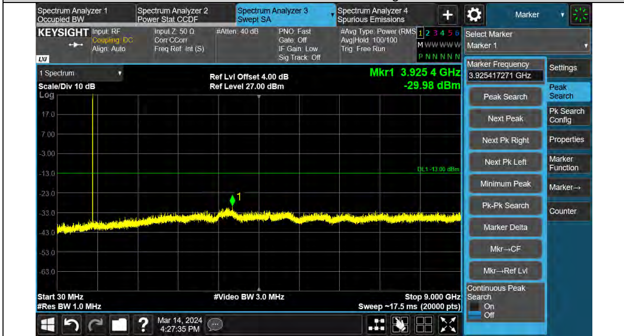
Band26-1.4MHz-QPSK-26783-1RB#0-Range:30~9000MHz
