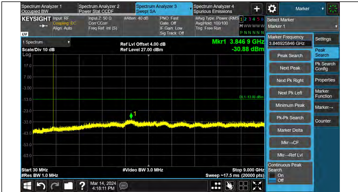
Band26-3MHz-16QAM-26705-1RB#0-Range:30~9000MHz
