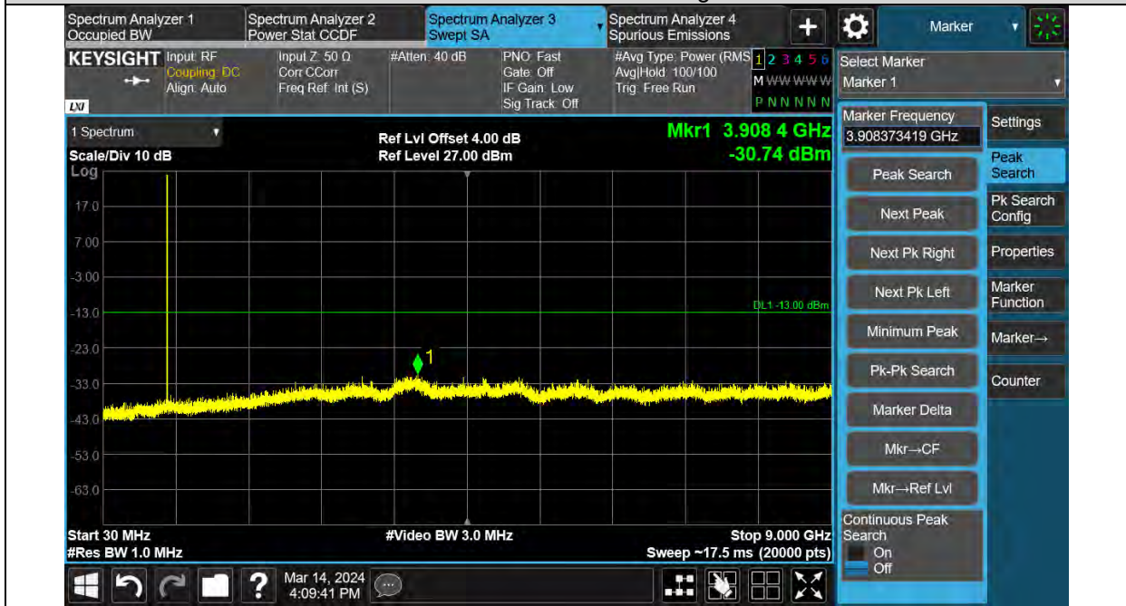
Band26-3MHz-QPSK-26775-1RB#0-Range:30~9000MHz
