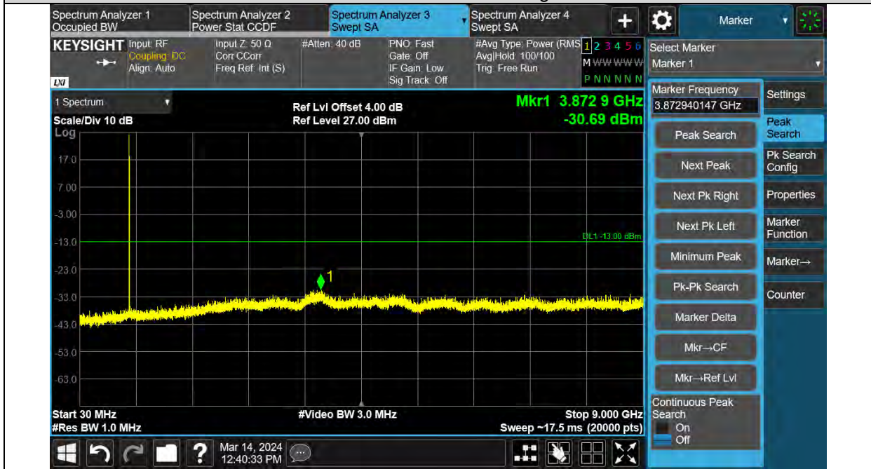
Band26-5MHz-QPSK-26765-1RB#0-Range:30~9000MHz
