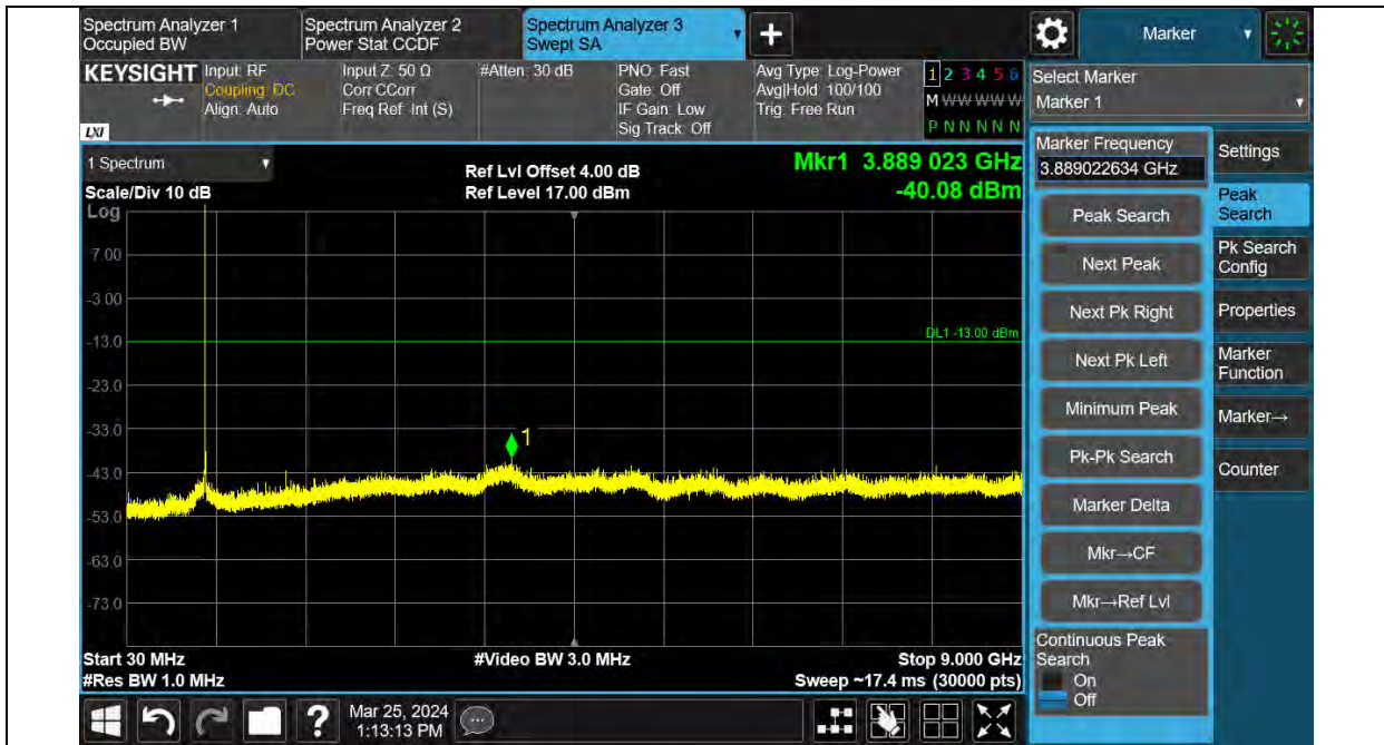
Band26-BPSK-3.75KHz-26740-1RB#0
