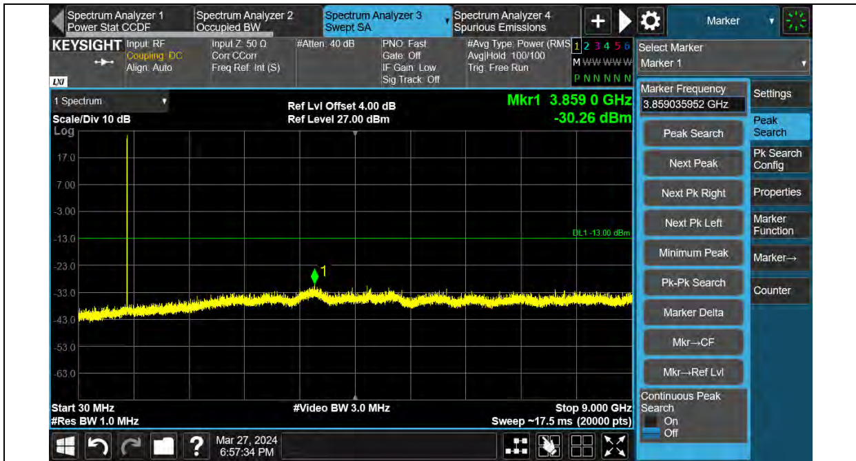
Band26-1.4MHz-16QAM-26783-1RB#0-Range:30~9000MHz
