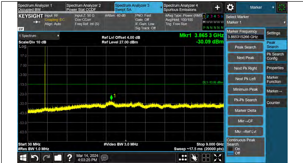
Band26-5MHz-16QAM-26715-1RB#0-Range:30~9000MHz
