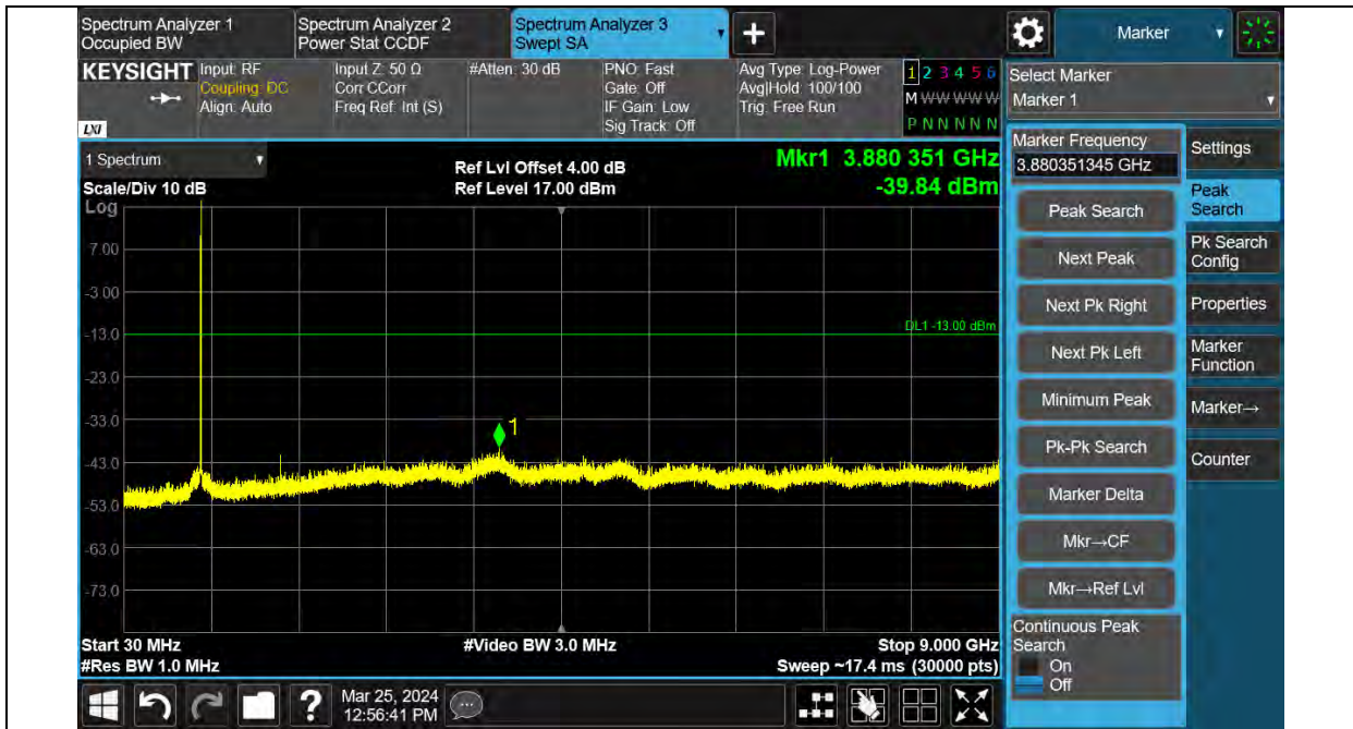
Band26-QPSK-3.75KHz-26788-1RB#0
