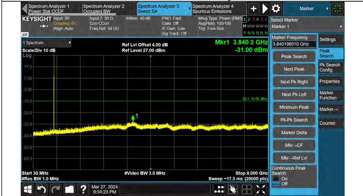
Band 26-10MHz-QPSK-26740-1RB#0-Range:30~9000MHz
