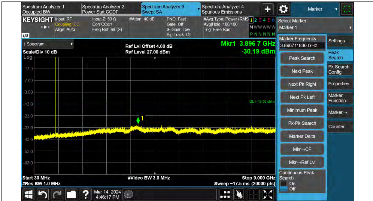
Band26-1.4MHz-16QAM-26697-1RB#0-Range:30~9000MHz
