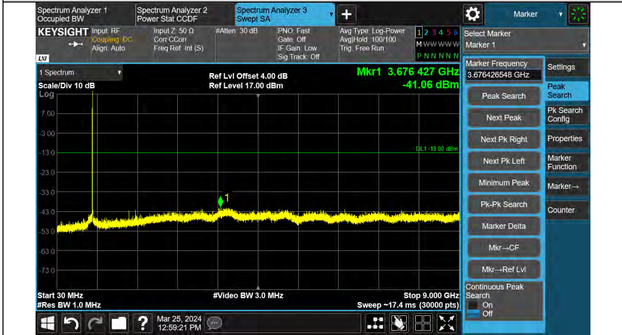
Band26-BPSK-3.75KHz-26788-1RB#0
