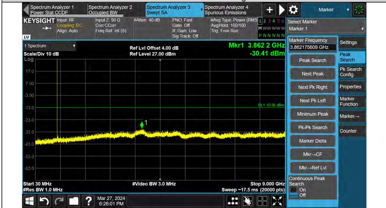
Band26-5MHz-16QAM-26740-1RB#0-Range:30~9000MHz
