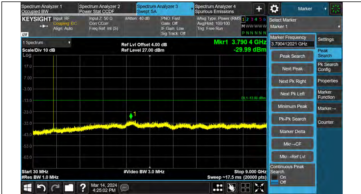
Band26-3MHz-QPSK-26740-1RB#0-Range:30~9000MHz
