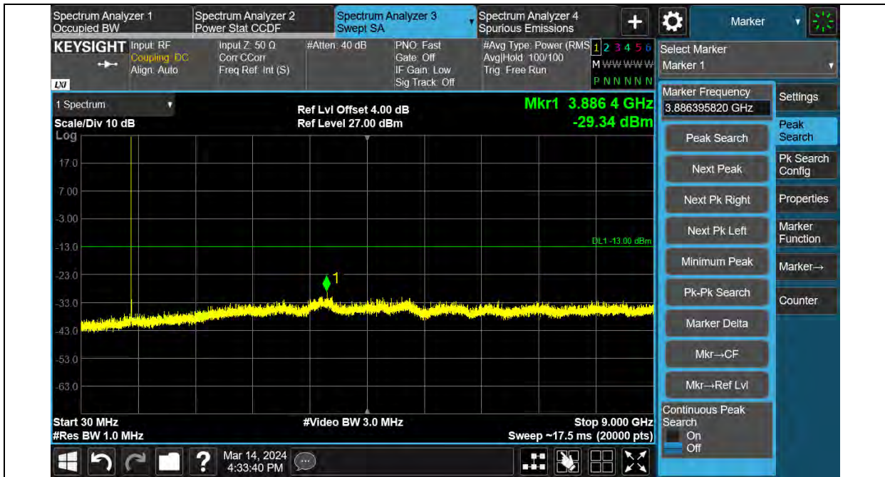
Band26-1.4MHz-QPSK-26740-1RB#0-Range:30~9000MHz
