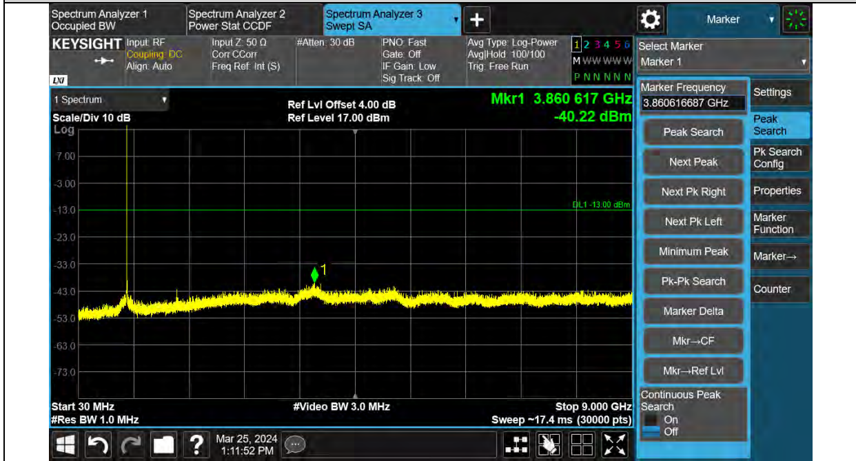
Band26-QPSK-3.75KHz-26740-1RB#0
