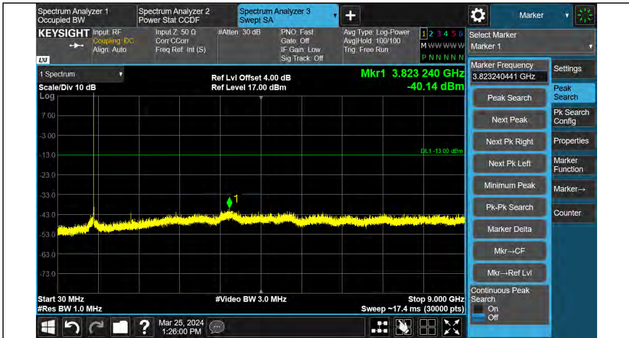
Band26-QPSK-3.75KHz-26692-1RB#0
