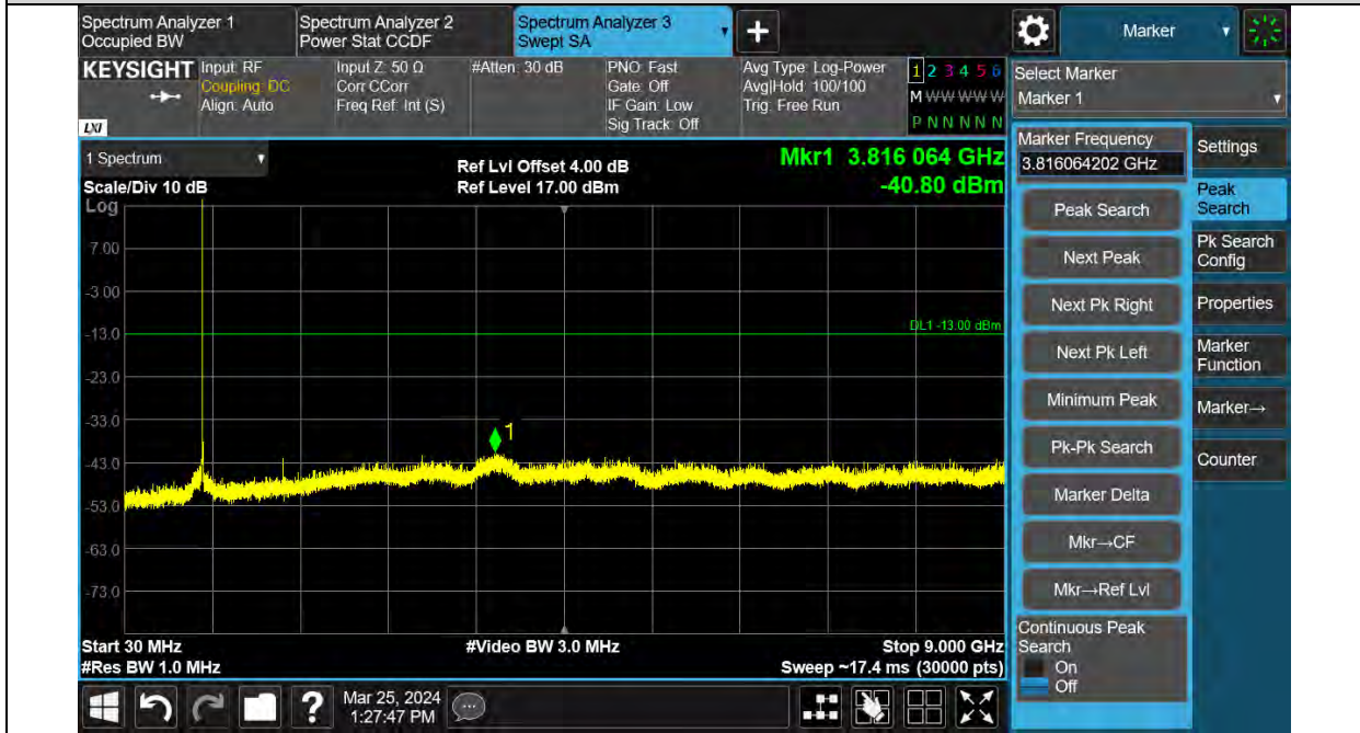
Band26-BPSK-15KHz-26692-1RB#0
