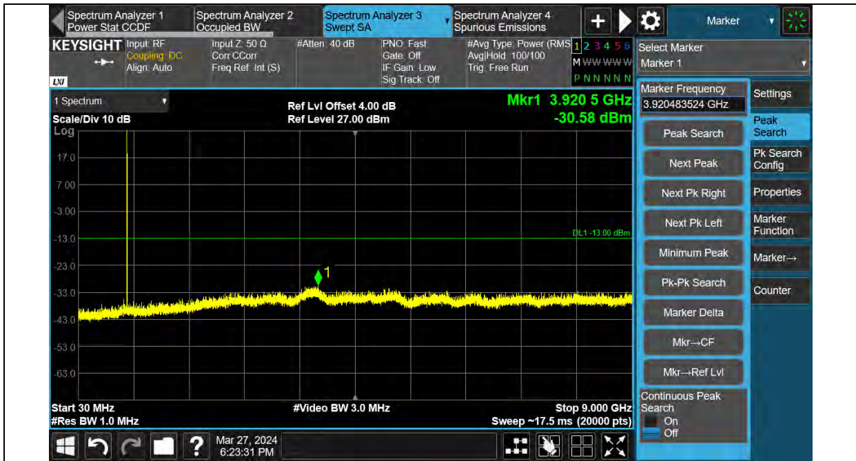
Band 26-5MHz-16QAM-26765-1RB#0-Range:30~9000MHz
