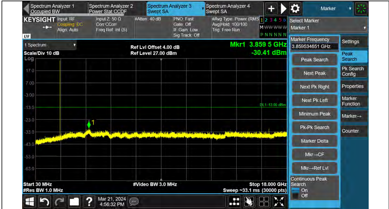
Band66-3MHz-16QAM-131987-1RB#0-Range:30~18000MHz
