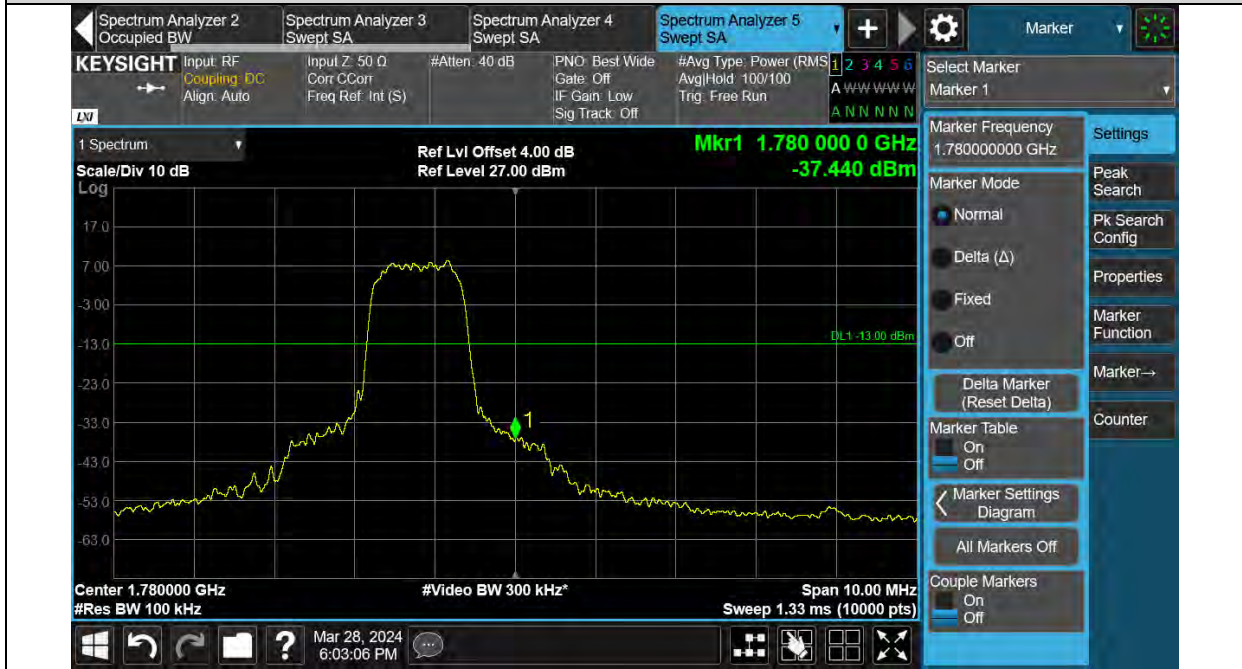
Band66-10MHz-16QAM-132022-1RB#0
