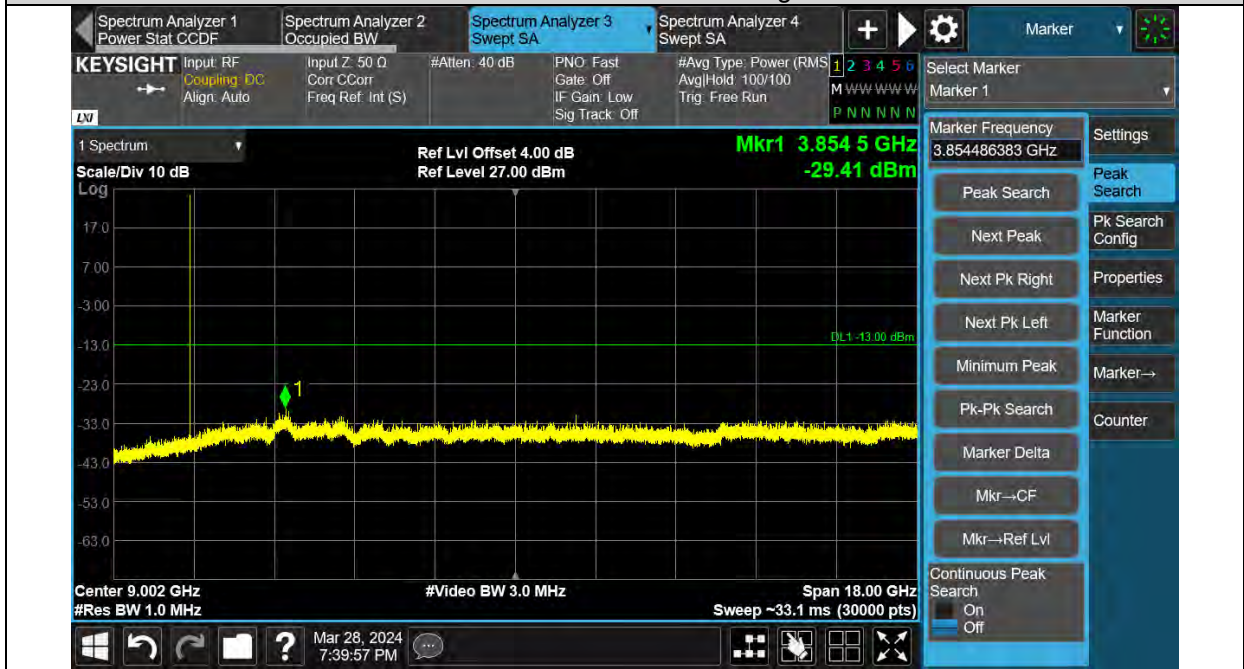
Band66-3MHz-16QAM-132322-1RB#0-Range:30~18000MHz
