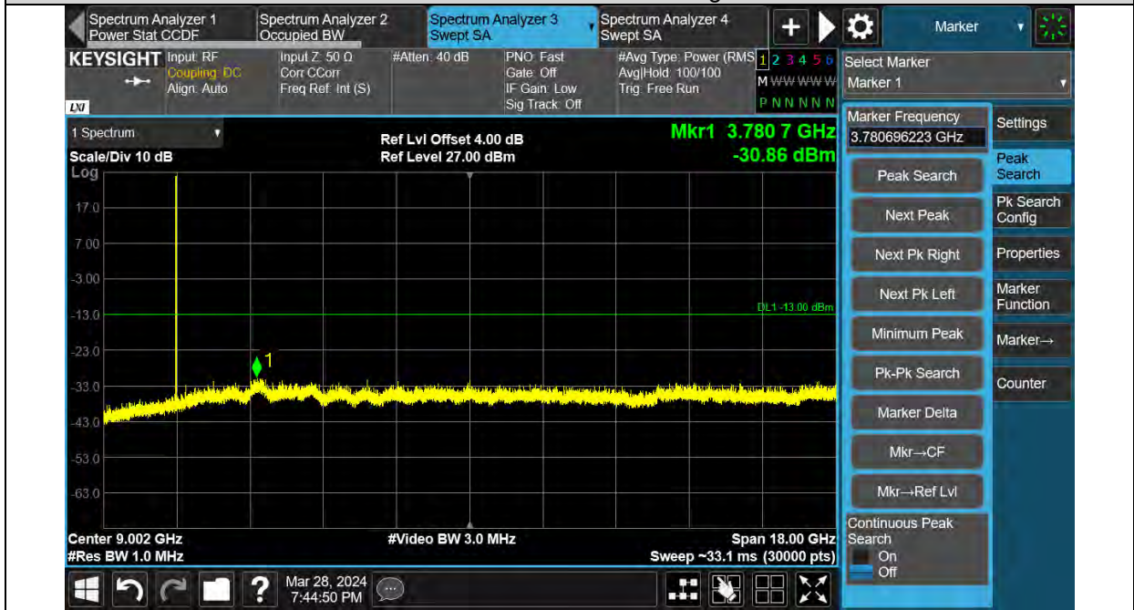
Band66-5MHz-QPSK-131997-1RB#0Range:30~18000MHz
