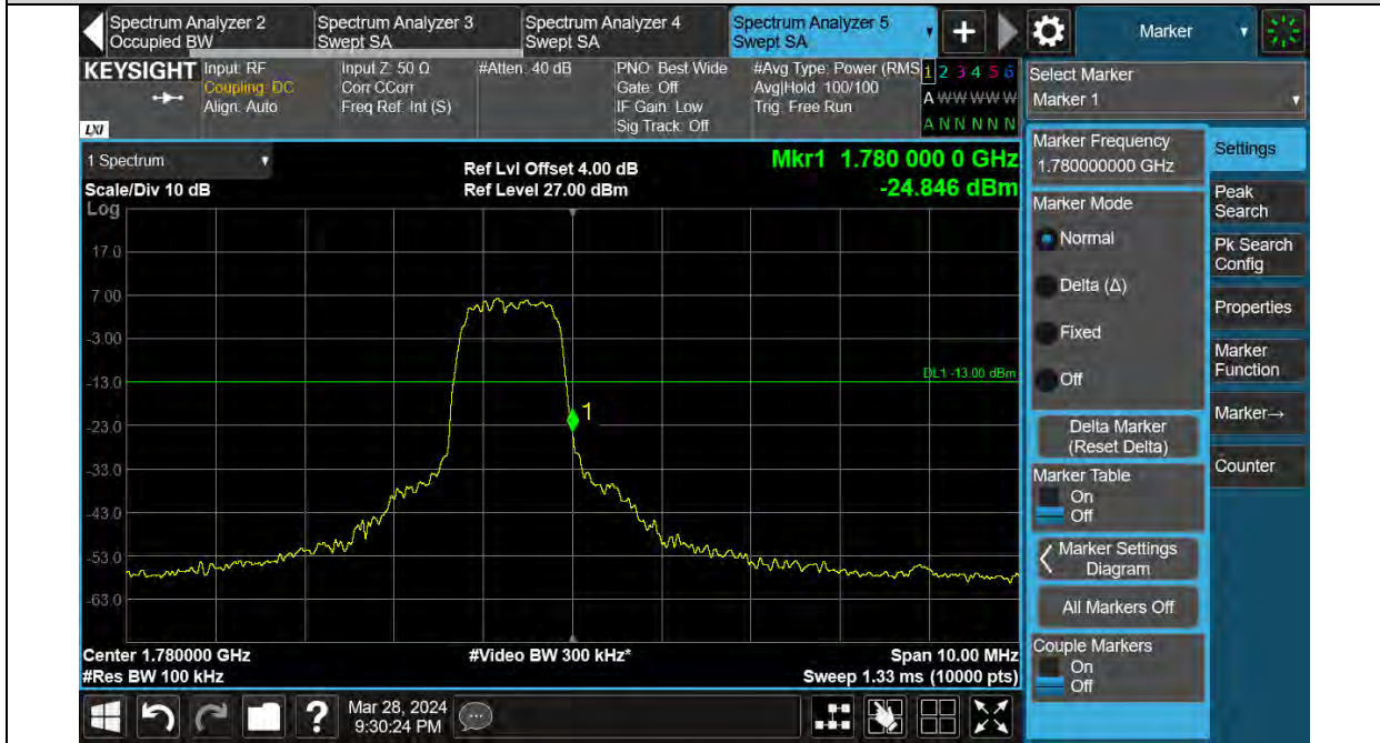
Band66-1.4MHz-16QAM-131979-1RB#0
