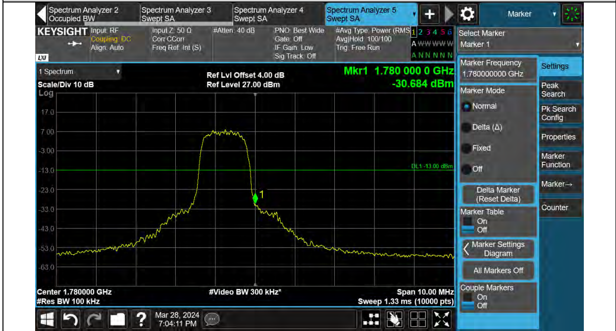
Band66-10MHz-QPSK-132022-1RB#0
