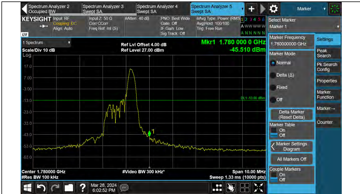
Band66-10MHz-QPSK-132622-6RB#0
