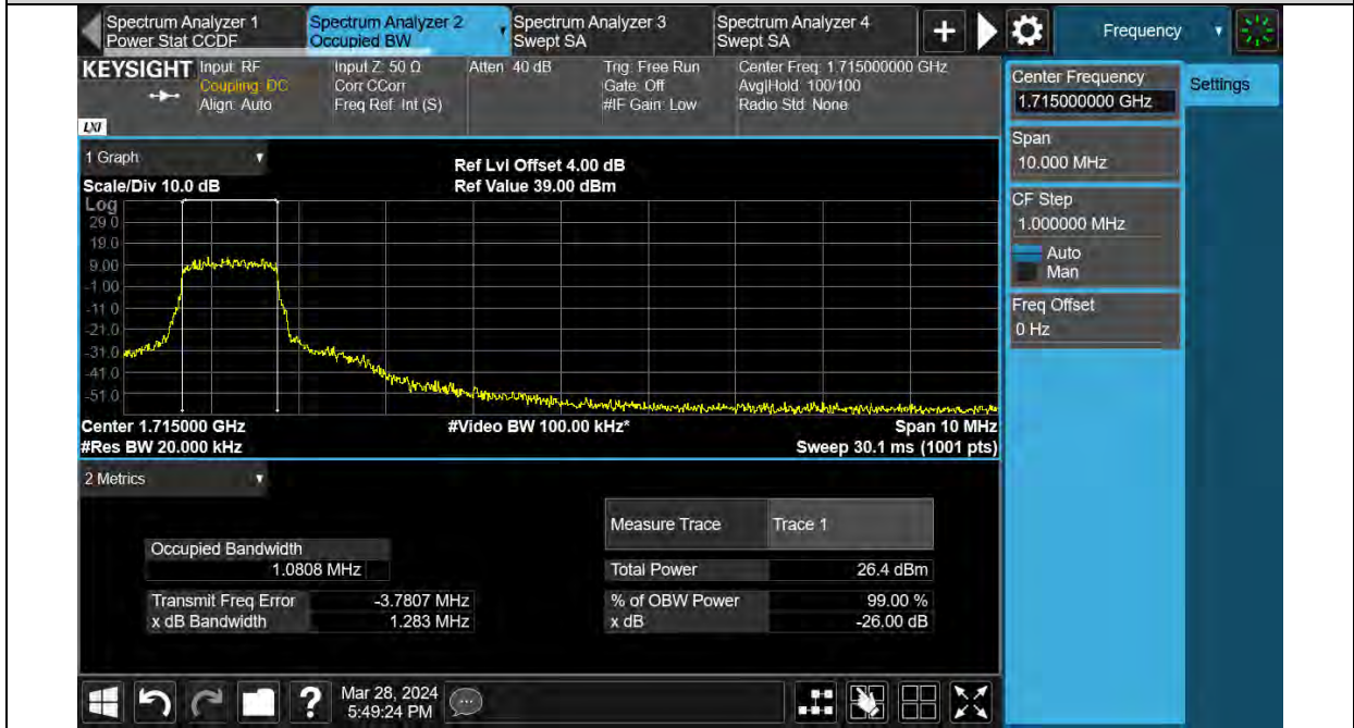
Band66-10MHz-QPSK-132322-6RB#0
