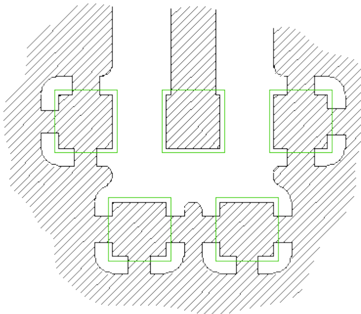
Figure 11: Layout for the Antenna pad connection
