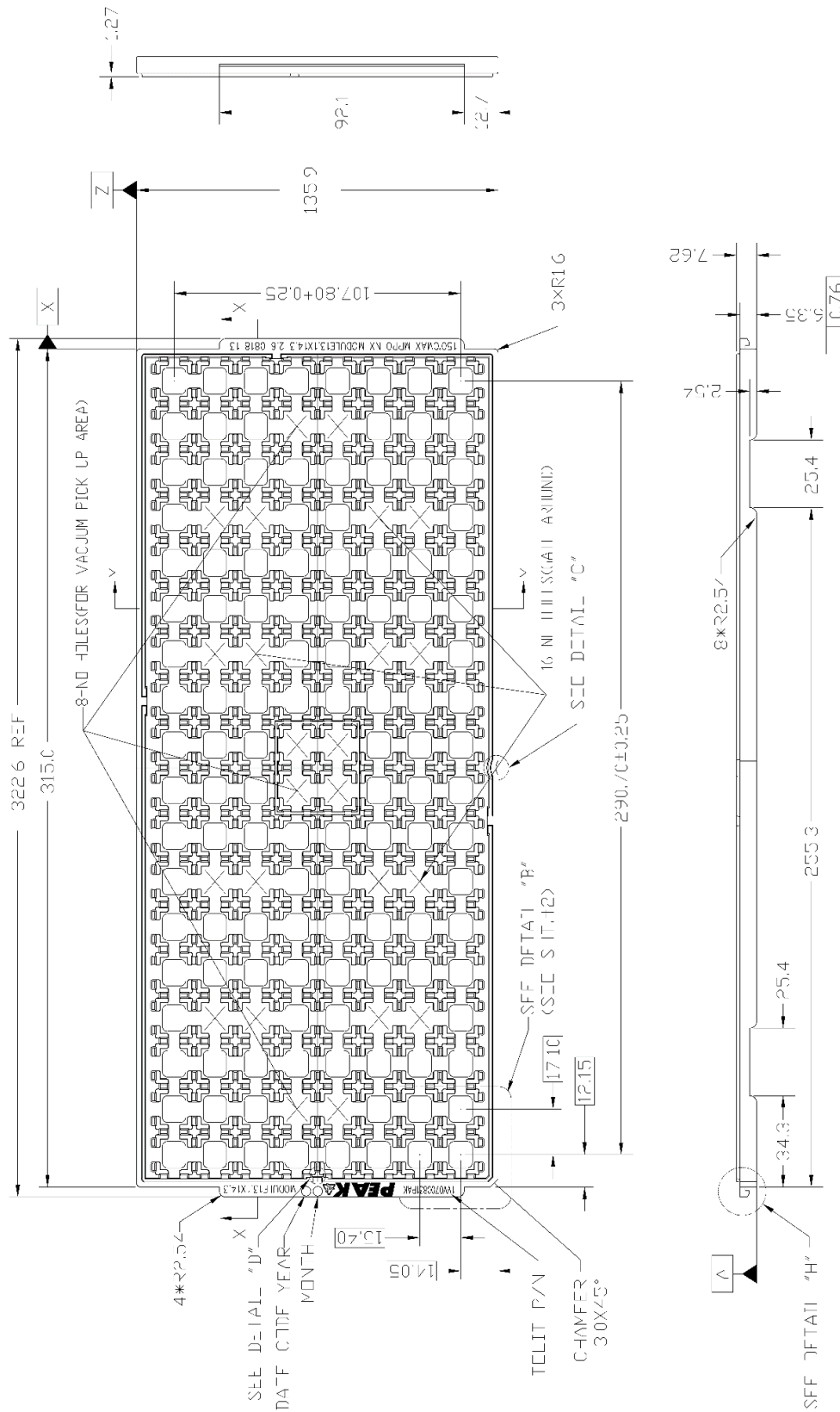
Figure 29: ME310G1-W1 tray
