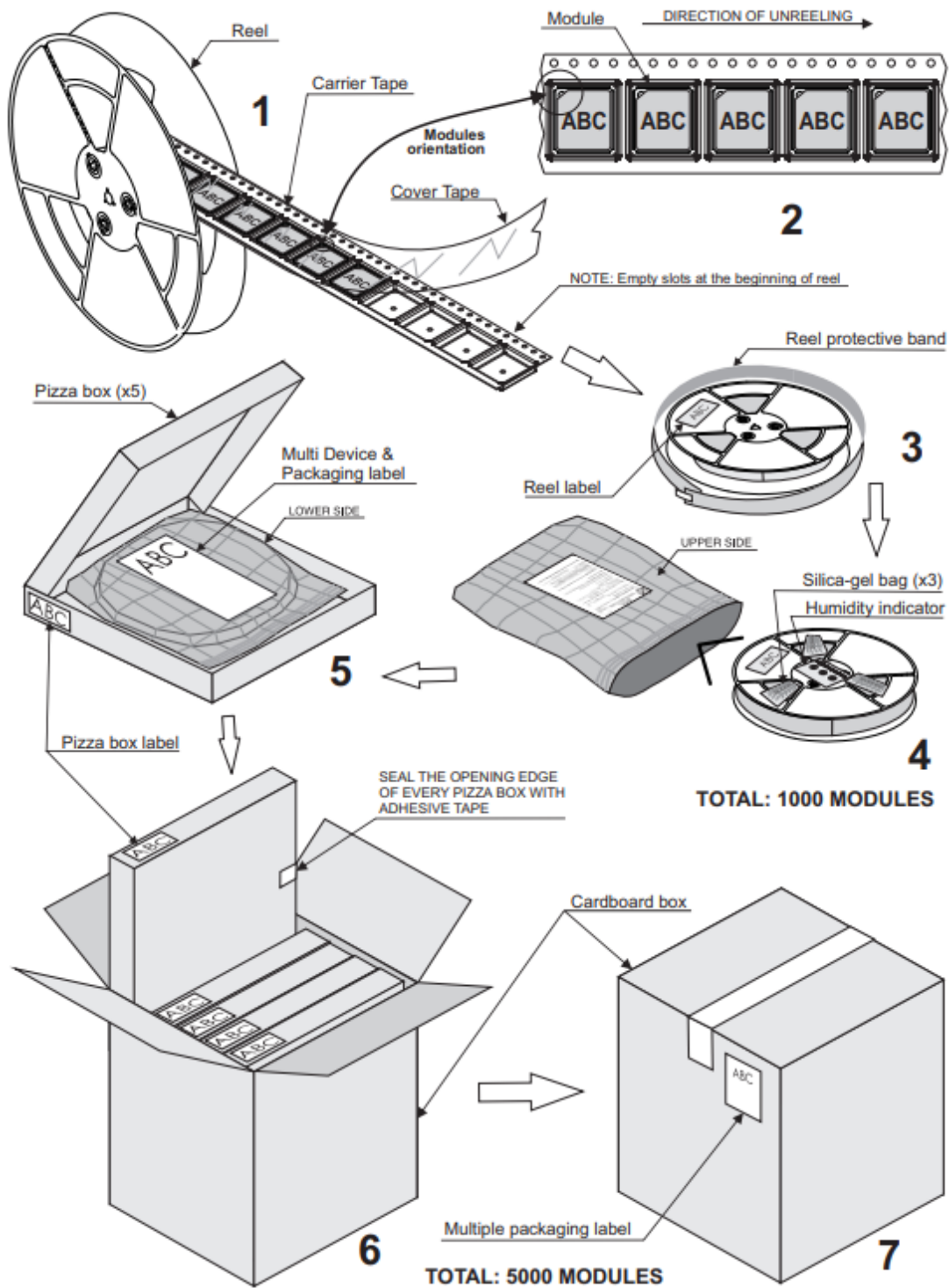
Figure 32: ME310G1-WW tray
