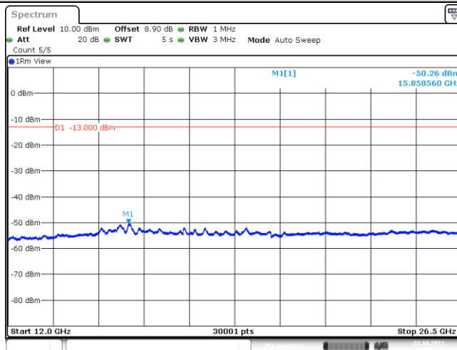
Band85-5MHz-QPSK-134157-1-5-High-12000-26500--50.26-PASS
