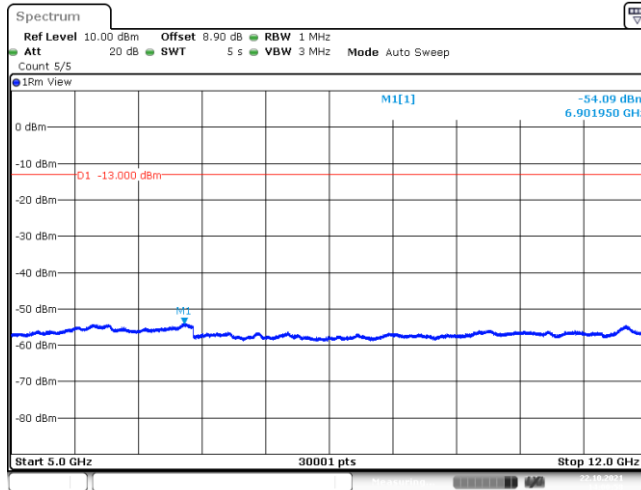
Band85-5MHz-QPSK-134157-1-5-High-5000-12000--54.09-PASS
