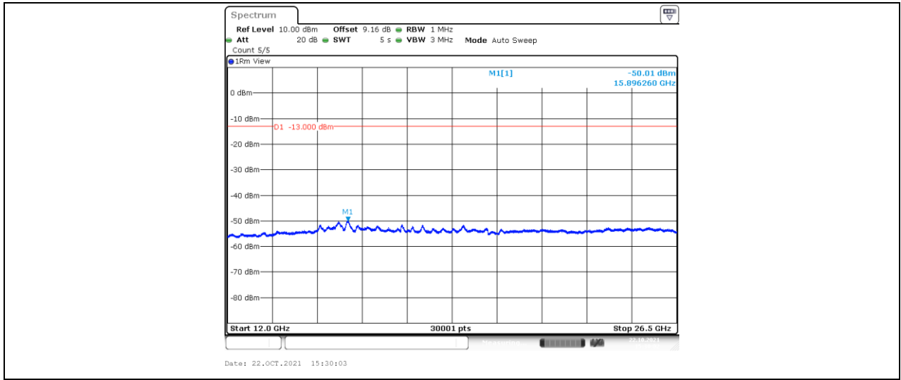
Band26-1.4MHz-16QAM-26915-6-0-Low-30-1000--34.96-PASS
