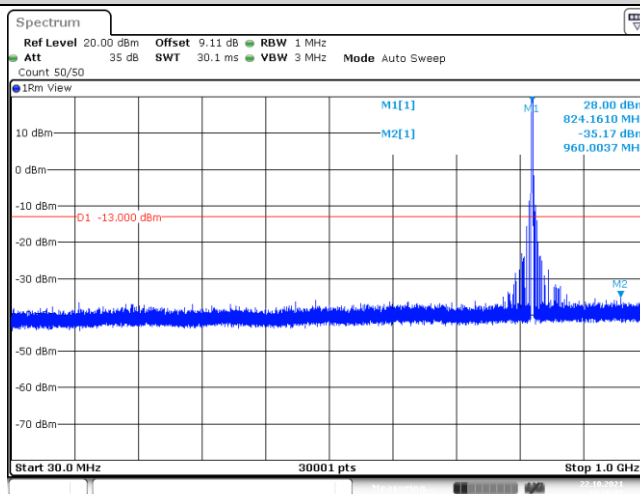
Band26-1.4MHz-QPSK-26797-1-0-Low-30-1000--35.17-PASS
