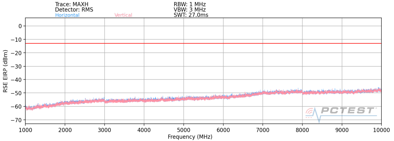
Plot 7-35. Radiated Spurious Plot (LTE Band 8- 3.75kHz SCS)
