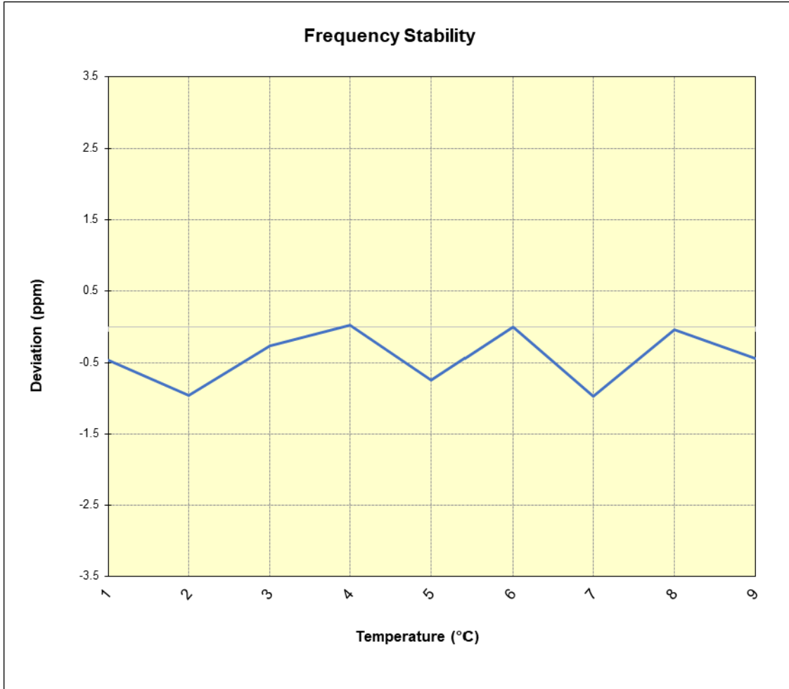
Plot 7-37. LTE Band 8 NB-IoT Frequency Stability Chart
