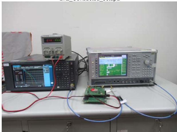
LTE_Conducted_setup2
